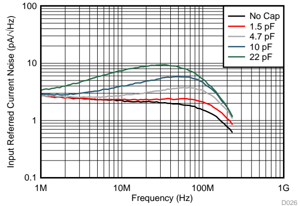
图 26. Input-Referred Current Noise Density vs Frequency
