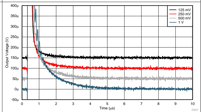
图 41. Long-Term Settling Response vs Output Voltage
