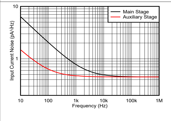
图 7-46. Input Current Noise Density vs Frequency
