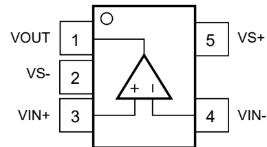
图 6-2. OPA863 DBV Package, 5-Pin SOT-23 (Top View)
