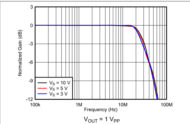
图 7-44. Frequency Response vs Supply Voltage
