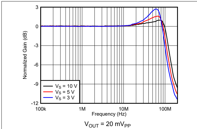
图 7-43. Frequency Response vs Supply Voltage
