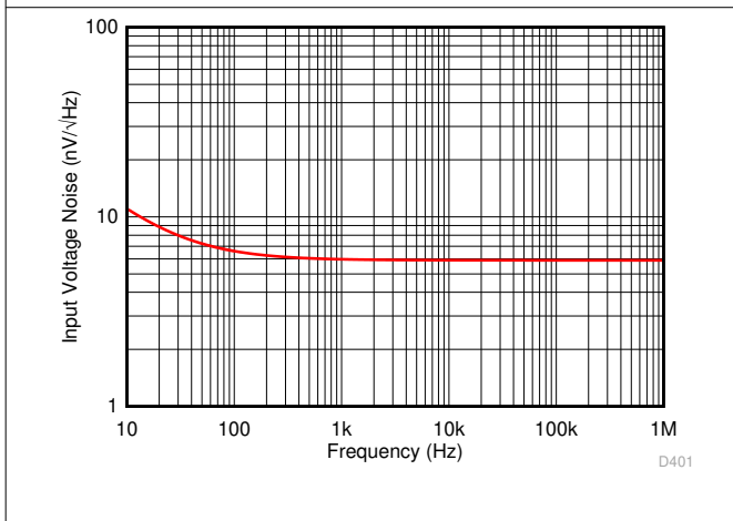
图 7-45. Input Voltage Noise Density vs Frequency
