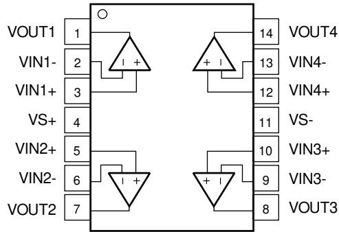
图 6-5. OPA4863 PW Package, 14-Pin TSSOP (Top View)
