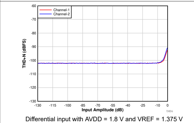
图 7-9. THD+N vs Input Amplitude With DRE Disabled
