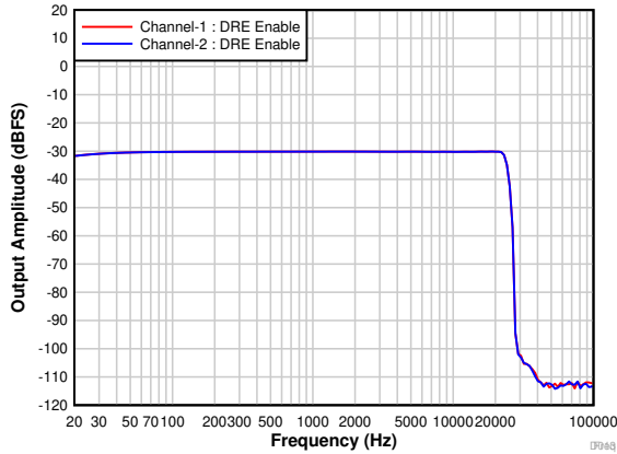
图 7-16. Frequency Response With a -30-dB Input
