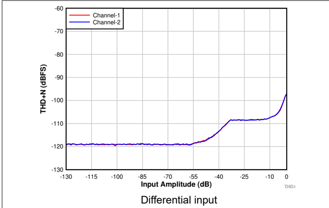
图 7-4. THD+N vs Input Amplitude With DRE Enabled
