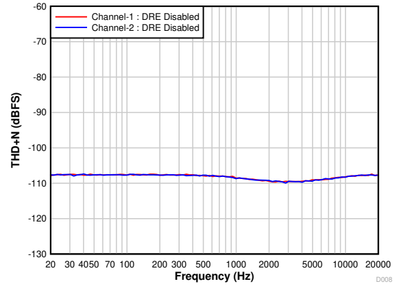
图 7-11. THD+N vs Input Frequency With a -60-dBr Input
