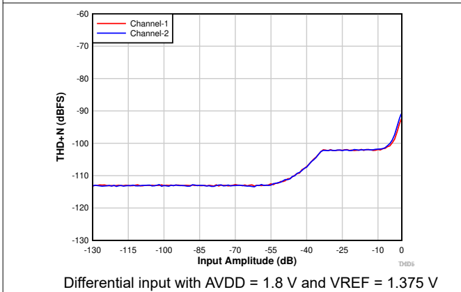
图 7-8. THD+N vs Input Amplitude With DRE Enabled
