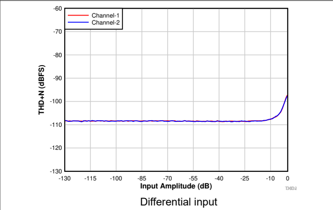
图 7-5. THD+N vs Input Amplitude With DRE Disabled
