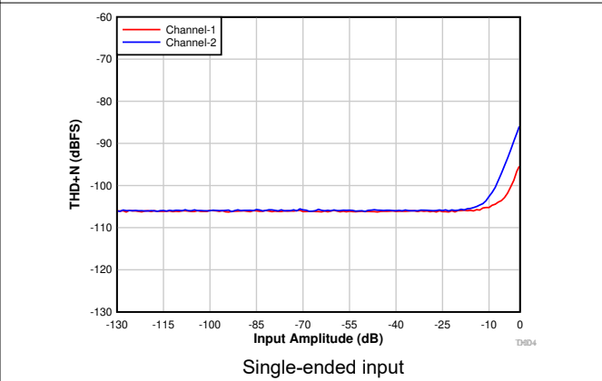
图 7-7. THD+N vs Input Amplitude With DRE Disabled
