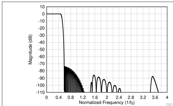
图 8-29. Linear Phase Decimation Filter Magnitude Response
