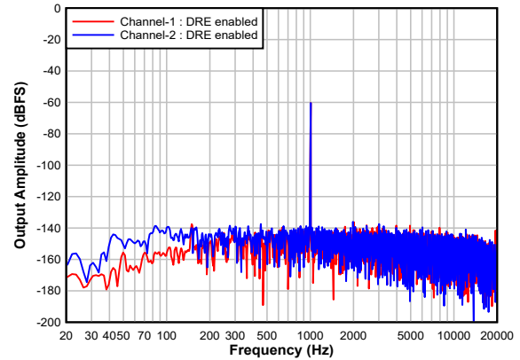
图 7-23. Single Ended FFT With a -60-dBr Input With DRE Enabled
