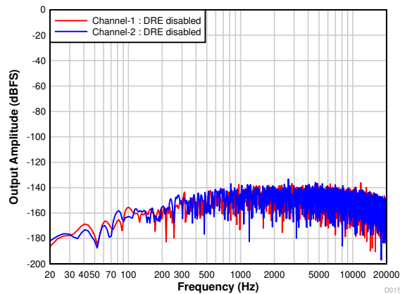
图 7-18. Differential FFT With Idle Input With DRE Disabled
