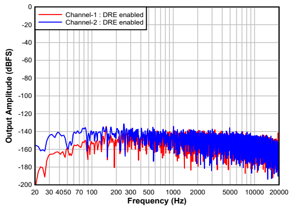
图 7-21. Single Ended FFT With Idle Input With DRE Enabled
