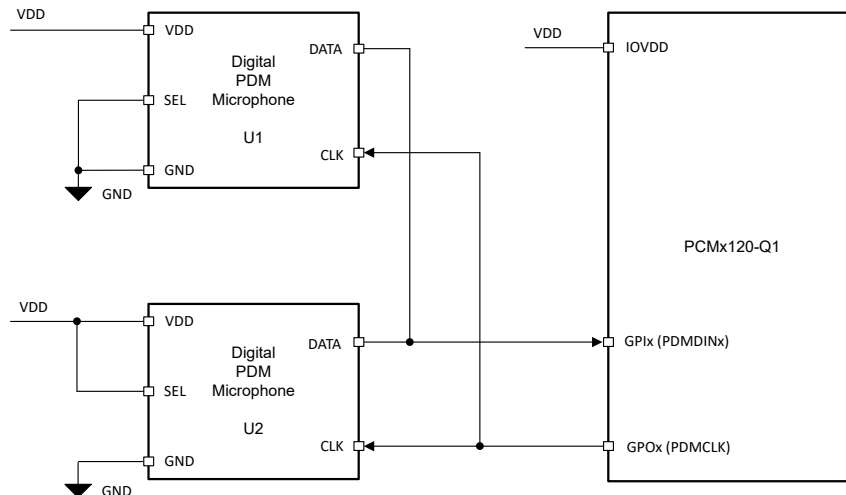
图 8-64. Digital PDM Microphones Connection Diagram for the PCM6120-Q1
