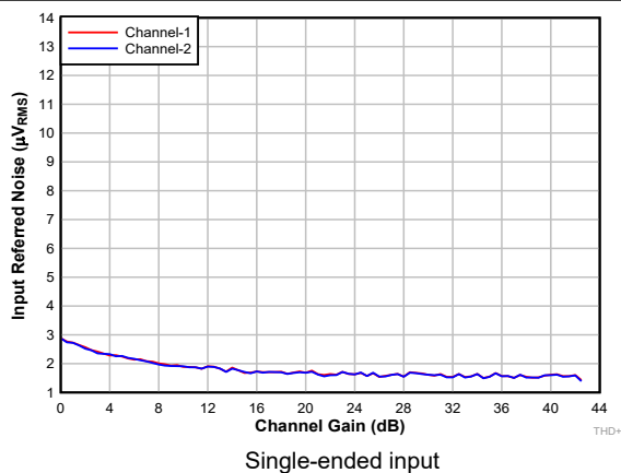
图 7-14. Input-Referred Noise vs Channel Gain
