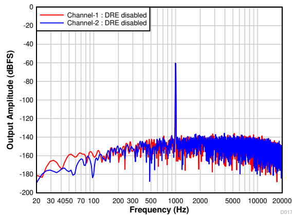
图 7-20. Differential FFT With a -60-dBr Input With DRE Disabled
