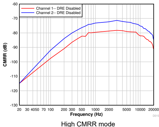
图 7-26. Common-Mode Rejection Ratio vs Ripple Frequency With 100-mV pp Amplitude and DRE Disabled
