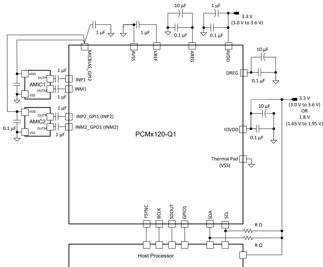
图 9-1. Two-Channel Analog Microphone Recording Diagram
