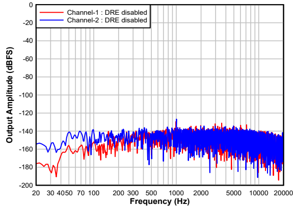
图 7-22. Single Ended FFT With Idle Input With DRE Disabled
