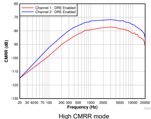
图 7-27. Common-Mode Rejection Ratio vs Ripple Frequency With 100-mV pp Amplitude and DRE Enabled
