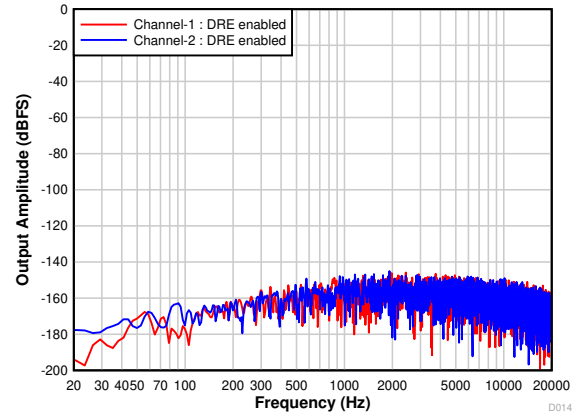
图 7-17. Differential FFT With Idle Input With DRE Enabled
