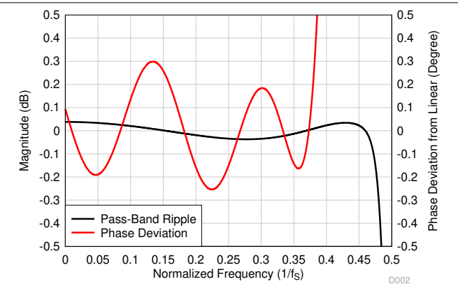
图 8-46. Low-Latency Decimation Filter Pass-Band Ripple and Phase Deviation
