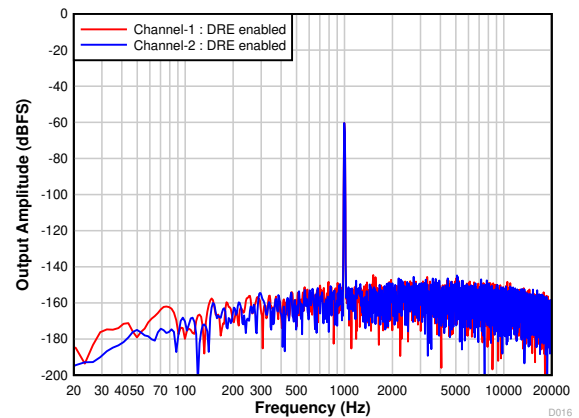
图 7-19. Differential FFT With a -60-dBr Input With DRE Enabled
