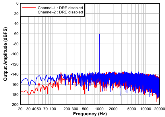
图 7-24. Single Ended FFT With a -60-dBr Input With DRE Disabled
