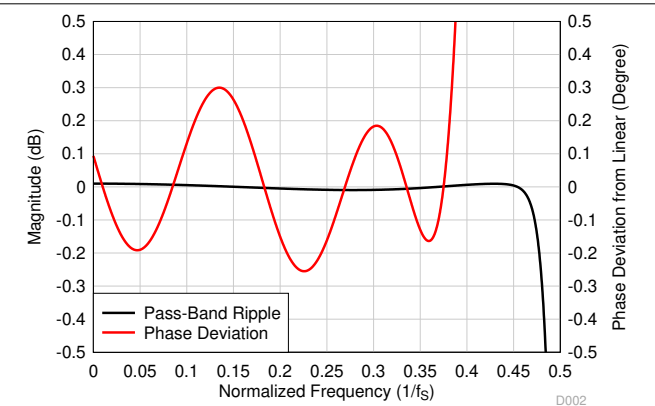
图 8-40. Low-Latency Decimation Filter Pass-Band Ripple and Phase Deviation
