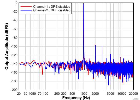
图 7-25. Differential FFT With a -1-dBr Input With DRE Disabled
