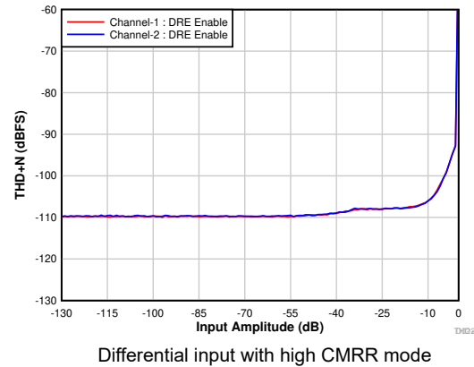
图 7-29. THD+N vs Input Amplitude With DRE Enabled
