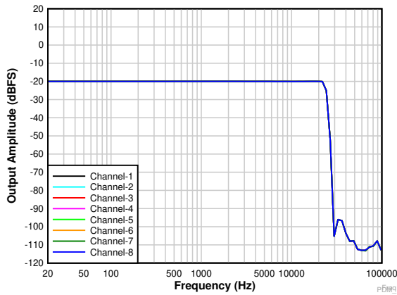
PDMCLKx = 3.072MHz 的四阶 PDM 调制器
