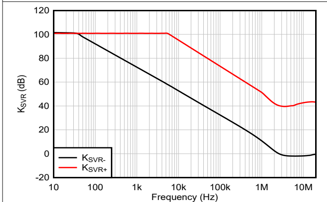
图 5-3. Supply Voltage Sensitivity vs Frequency
