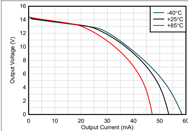
图 5-17. Output Voltage Swing vs Output Current (Sourcing)
