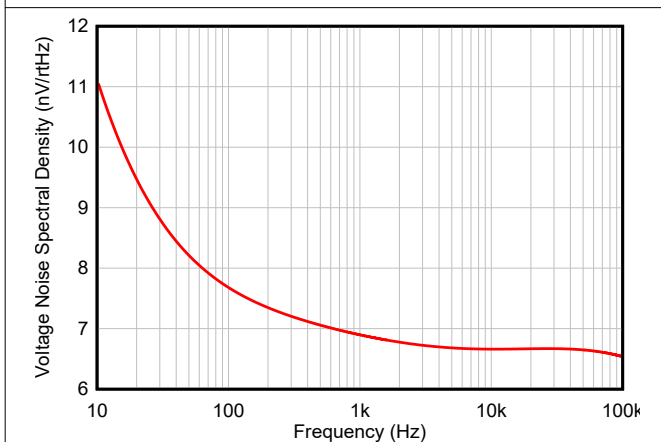
图 5-5. Input Noise Voltage vs Frequency
