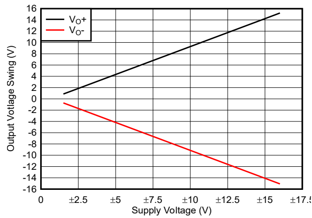
图 5-16. Maximum Output Voltage Swing vs Operating Voltage
