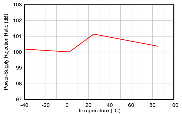
图 5-24. Power Supply Rejection Ratio vs Temperature
