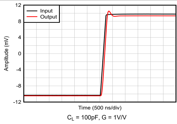
图 5-14. Small Signal Step Response
