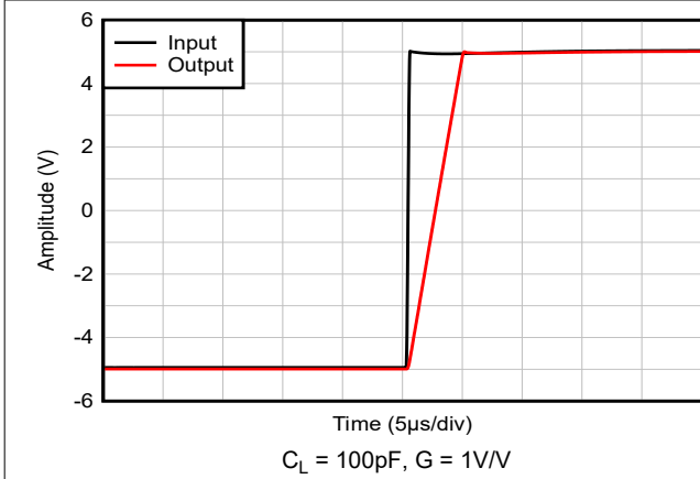
图 5-13. Large Signal Step Response
