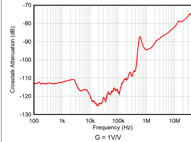
图 5-15. Crosstalk Attenuation vs Frequency
