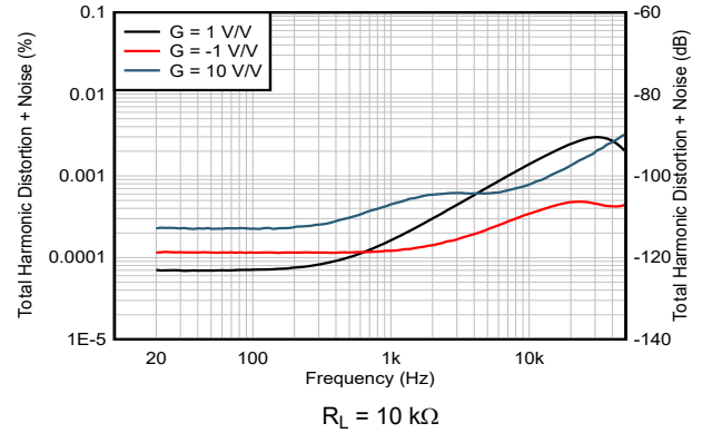
图 5-8. THD+N vs Frequency
