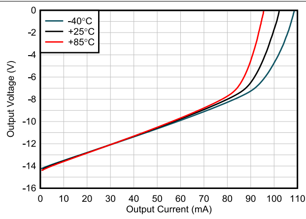
图 5-18. Output Voltage Swing vs Output Current (Sinking)
