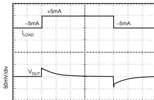
200 \mu\text{s}/\text{div} C_L = 1\text{ }\mu\text{F} , \pm 5\text{mA} 输出脉冲
