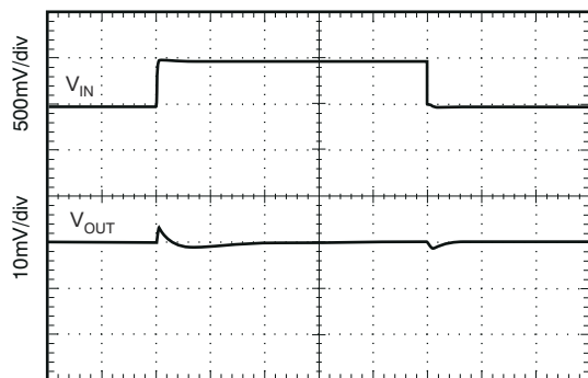
Time (200 \mu\text{s}/\text{div} ) C_{\text{LOAD}} = 10\text{ }\mu\text{F} , I_{\text{OUT}} = 1\text{mA}
