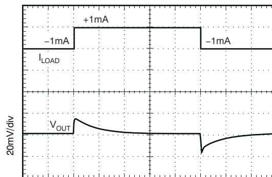
200 \mu\text{s}/\text{div} C_L = 1\text{ }\mu\text{F} , \pm 1\text{mA} 输出脉冲
