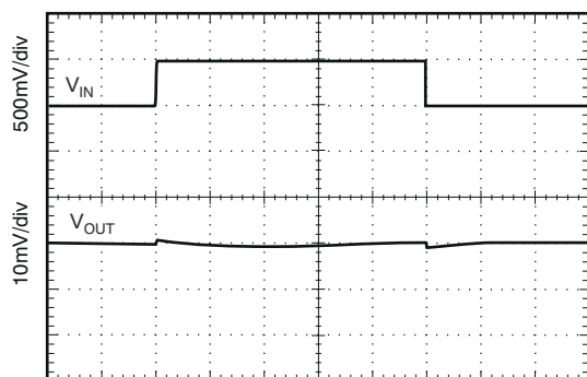
Time (400 \mu\text{s}/\text{div} ) C_{\text{LOAD}} = 10\text{ }\mu\text{F} , I_{\text{OUT}} = 0\text{mA}
