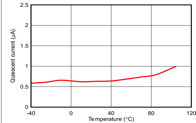
图 6-33. Quiescent Current vs Free-Air Temperature
