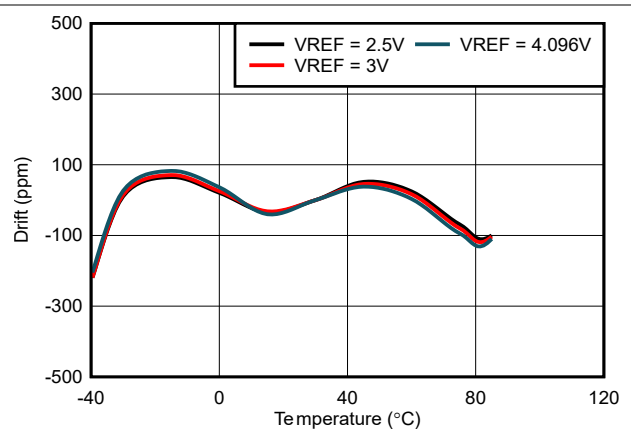
WCSP Package V_{REF} \geq 2.5\text{V} (-40°C to 85°C)
