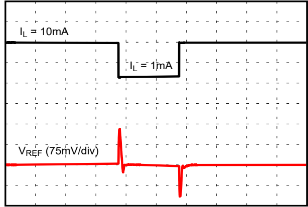
图 8-4. Load Transient Response 1mA to 10mA, C_L = 1 \mu F
