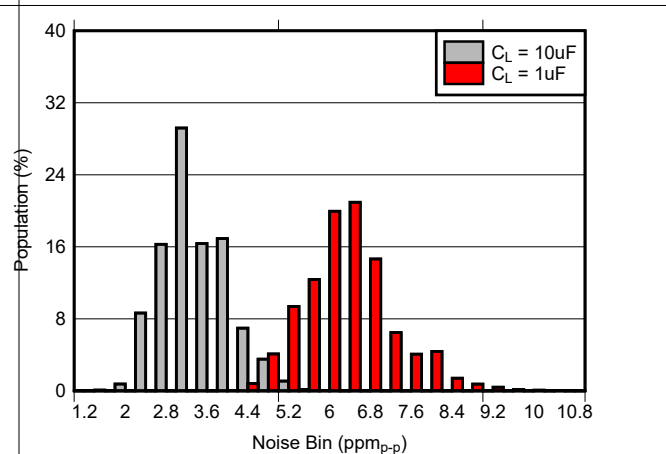
图 6-12. 0.1Hz to 10Hz Noise Distribution ( V_{REF} = 1.25\text{V} , C_{NR} = \text{Open} , I_L = 0\text{mA} )
