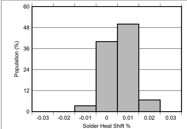
图 6-35. Solder Heat Shift Distribution
