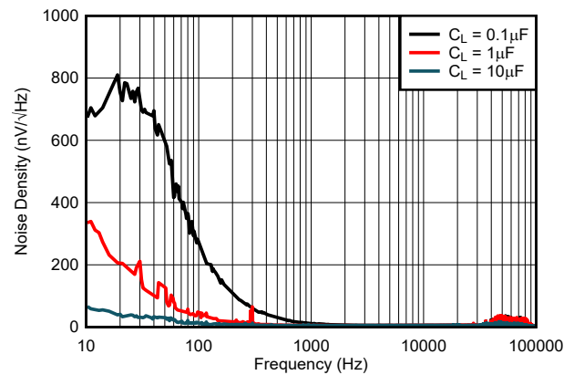
图 6-18. Noise Density vs Frequency ( V_{REF} = 2.5\text{V} , I_L = 0\text{mA} )
