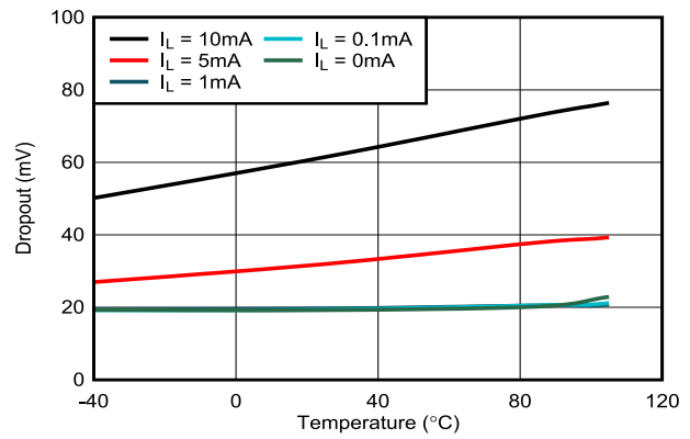
图 6-34. Dropout Voltage vs Free-Air Temperature
