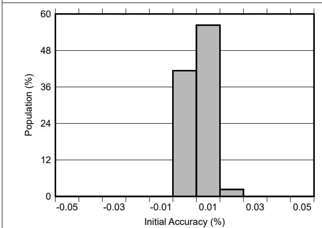
图 6-11. Initial Accuracy Distribution
