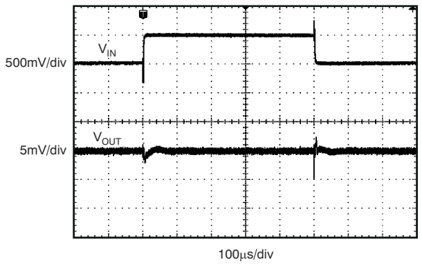
C_L = 10 \mu\text{F}
