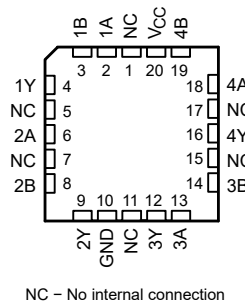
图 5-4. SN54AHC86 FK Package, LCCC 20-Pin (Top View)
