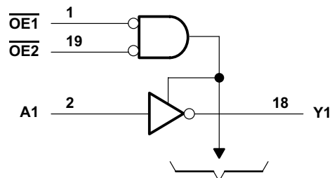
图 6-1. Logic Diagram (Positive Logic)
