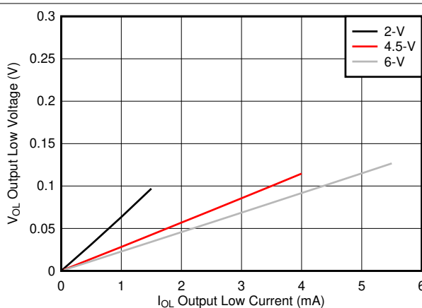
图 6-2. Typical output voltage in the low state ( V_{OL} )
