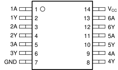
图 5-2. SN74LV6T07 PW Package, 14-Pin TSSOP (Top View)
