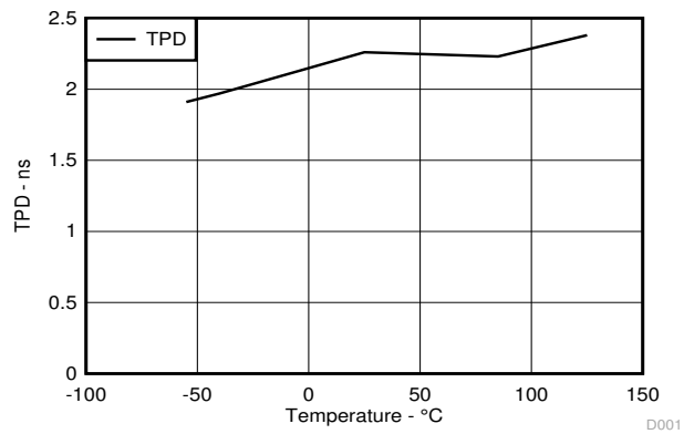
图 6-1. TPD Across Temperature at 3.3 V V CC
