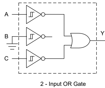
2 - Input OR Gate
