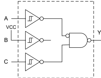
2 - Input NAND Gate with one inverted input
