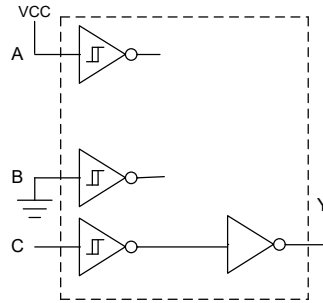
Inverter
