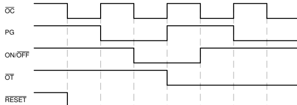
图 8-2. Typical Application Timing Diagram
