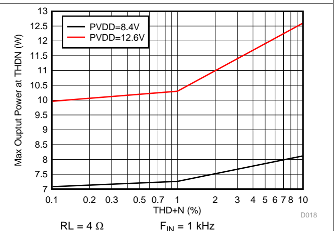
Figure 20. Max Output Power vs THD+N
