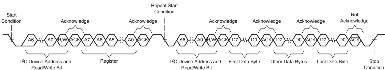
图 54. Multi-Byte Read Transfer
