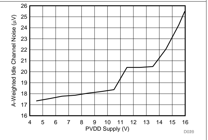
Figure 18. Idle Channel Noise (A-Weighted) vs PVDD
