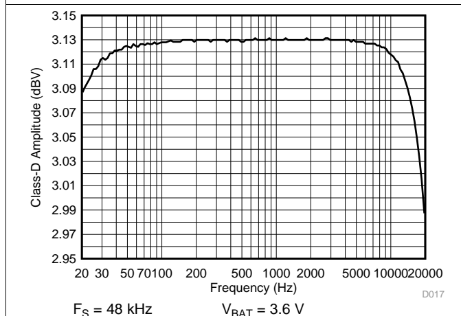
Figure 19. Amplitude vs Frequency
