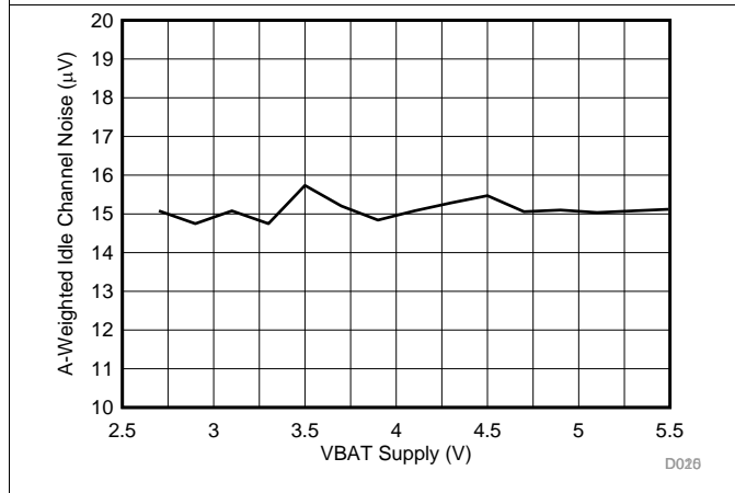
Figure 17. Idle Channel Noise (A-Weighted) vs VBAT
