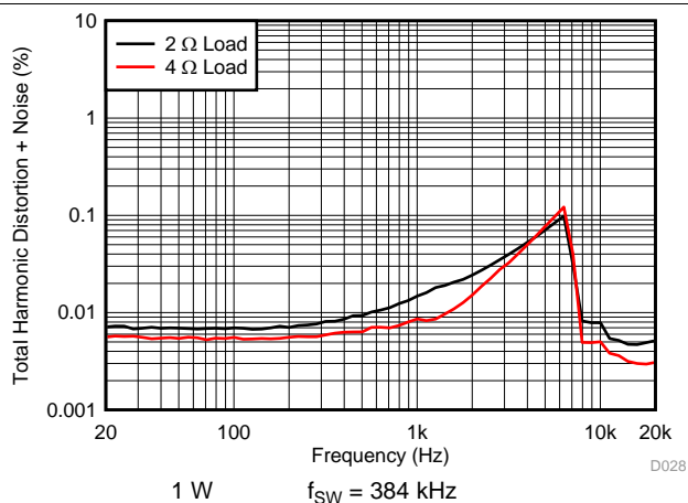
图 22. PBTL THD+N vs Frequency
