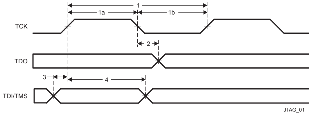
图 5-106. JTAG Timing
