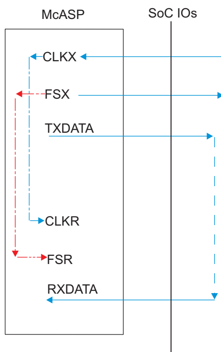
Figure 5-62. McASP1-8 CI-FO- – SYNC Mode
