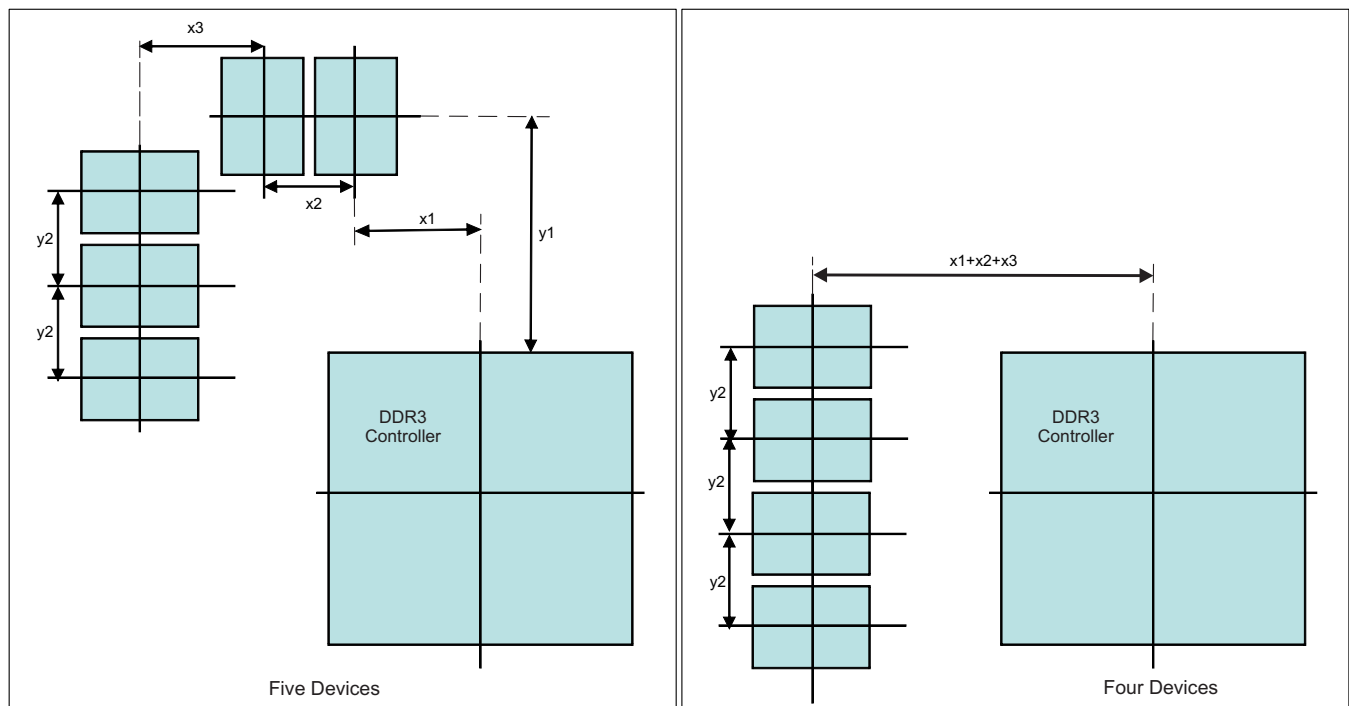
图 7-60. Placement Specifications
