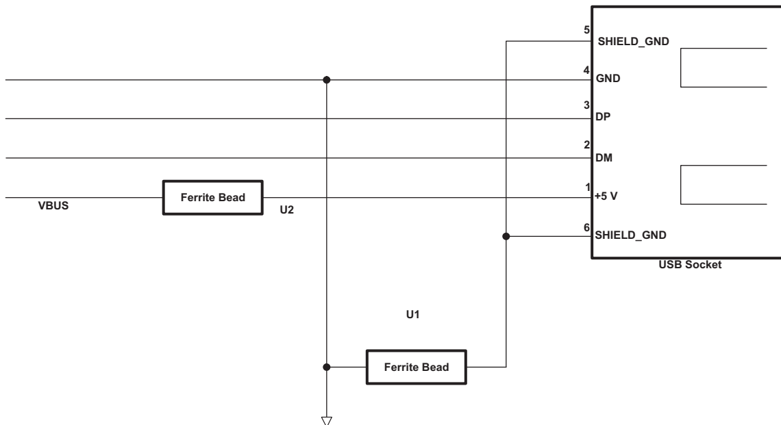
图 7-32. USB Connector
