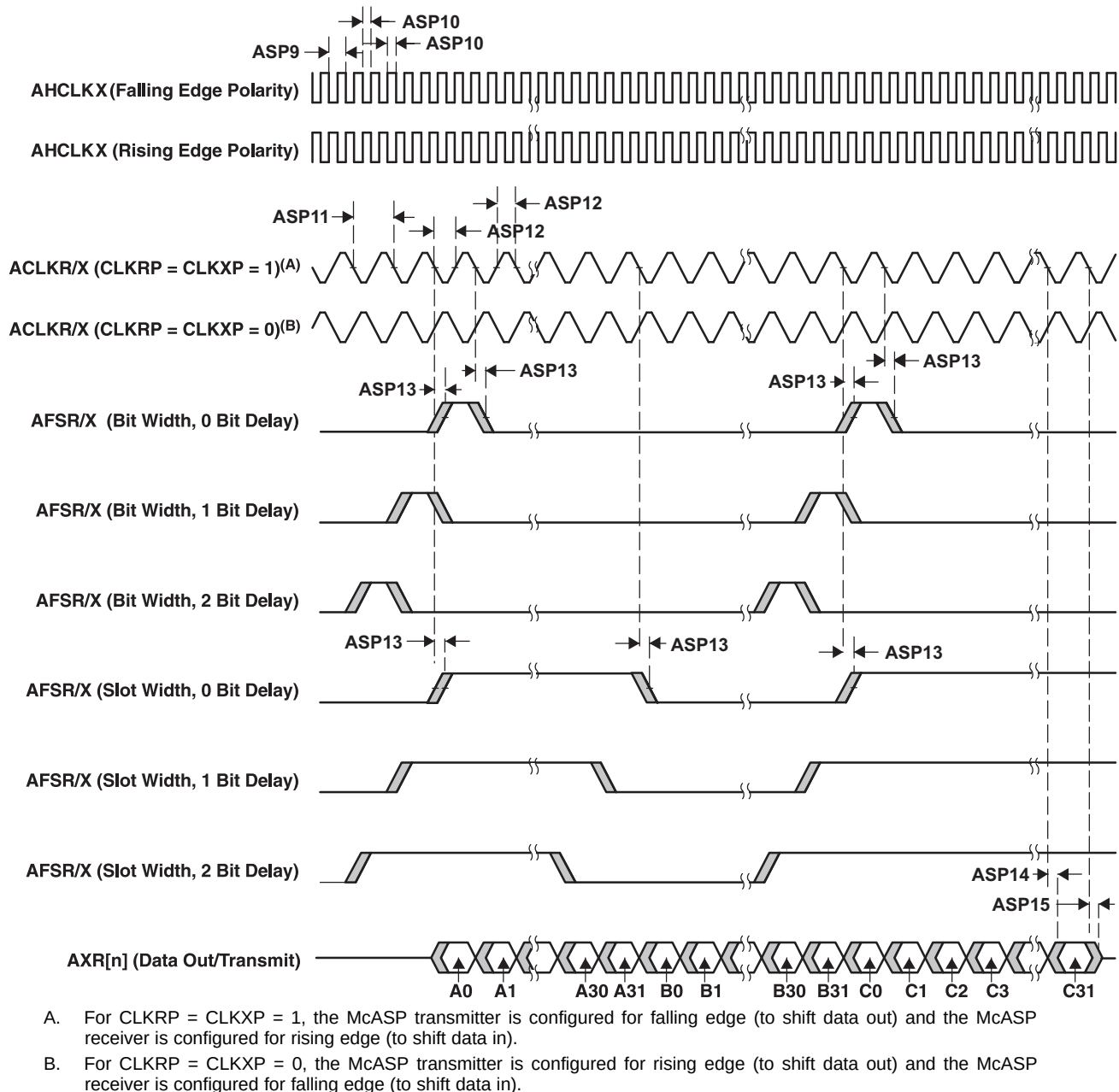
Figure 5-56. McASP Output Timing
