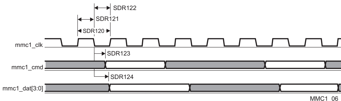
Figure 5-80. MMC/SD/SDIO in - High Speed SDR12 - Transmitter Mode
