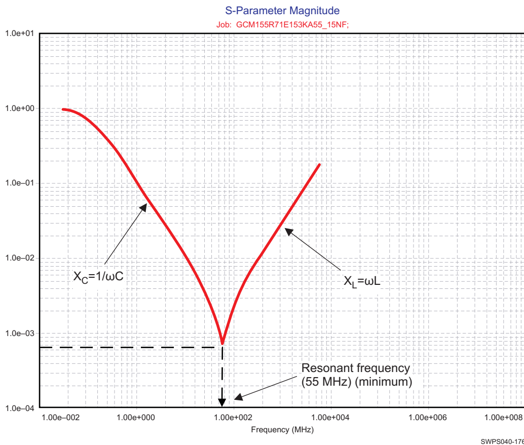
图 7-14. Typical Impedance Profile of a Capacitor
