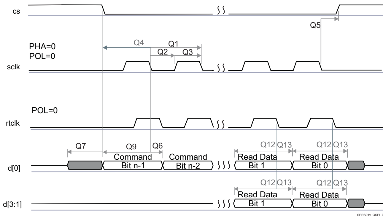
Figure 5-52. QSPI Read (Clock Mode 0)
