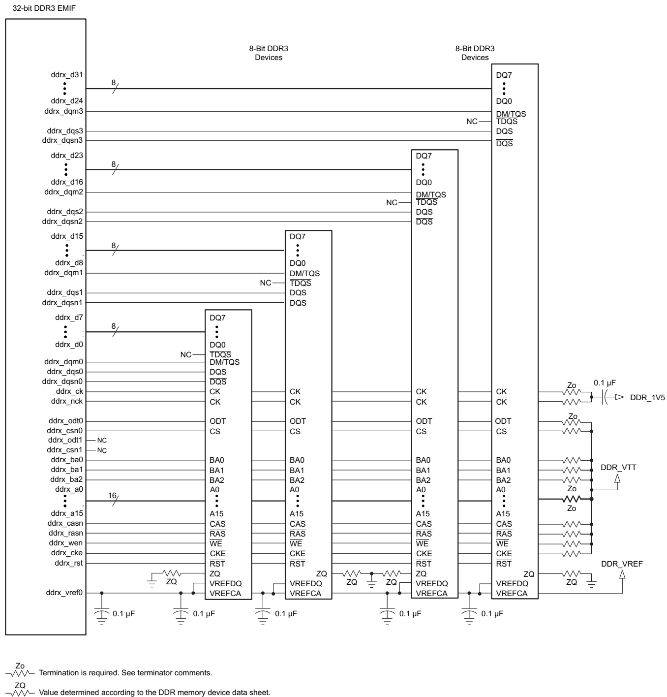
图 7-59. 32-Bit, One-Bank DDR3 Interface Schematic Using Four 8-Bit DDR3 Devices
