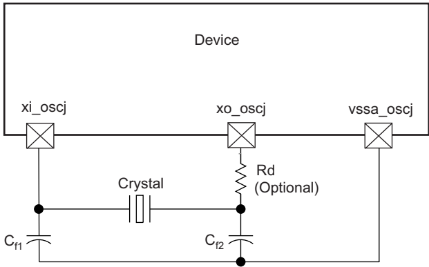
图 7-48. Grounding Scheme for High-Frequency Clock
