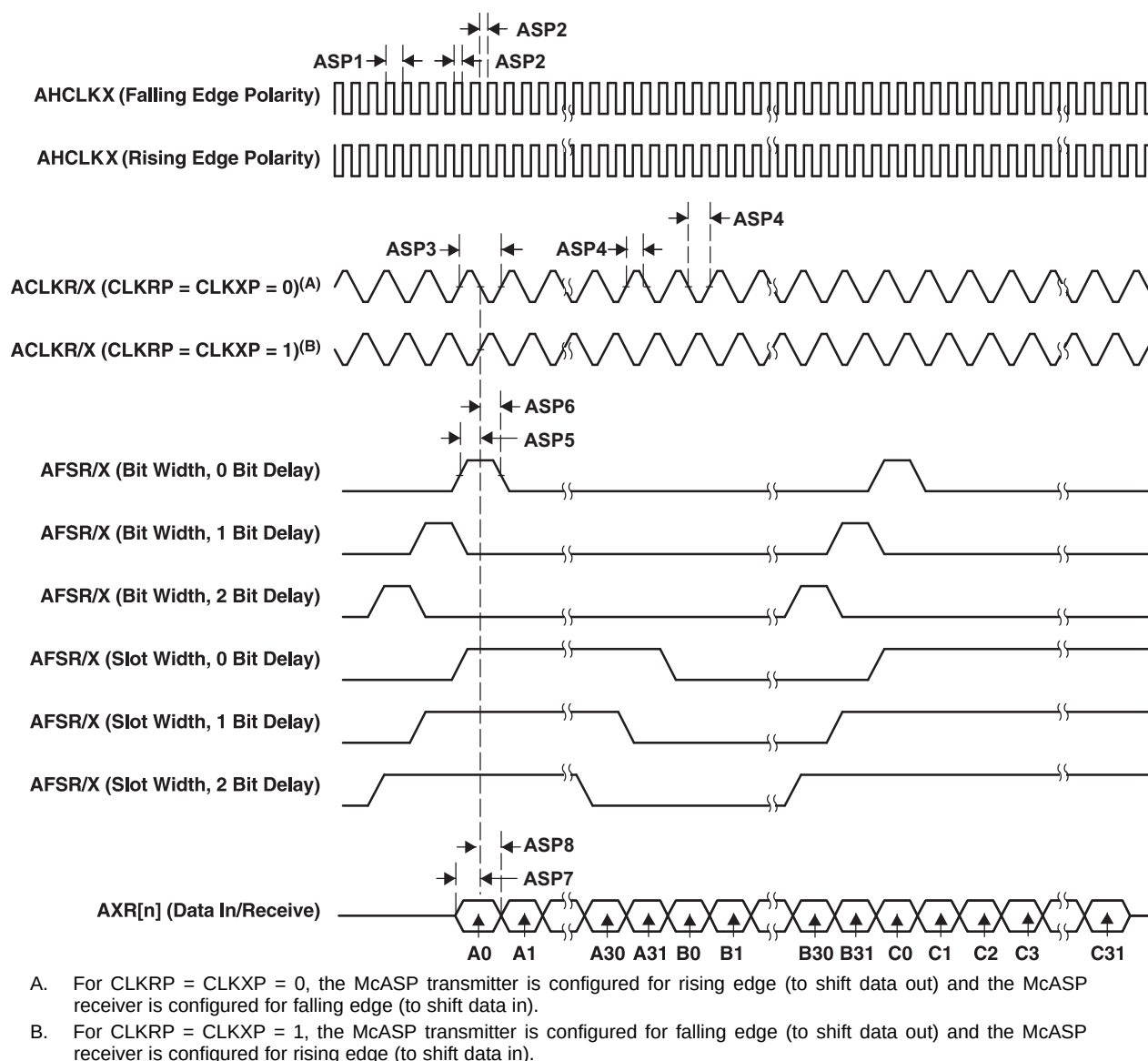
Figure 5-55. McASP Input Timing
