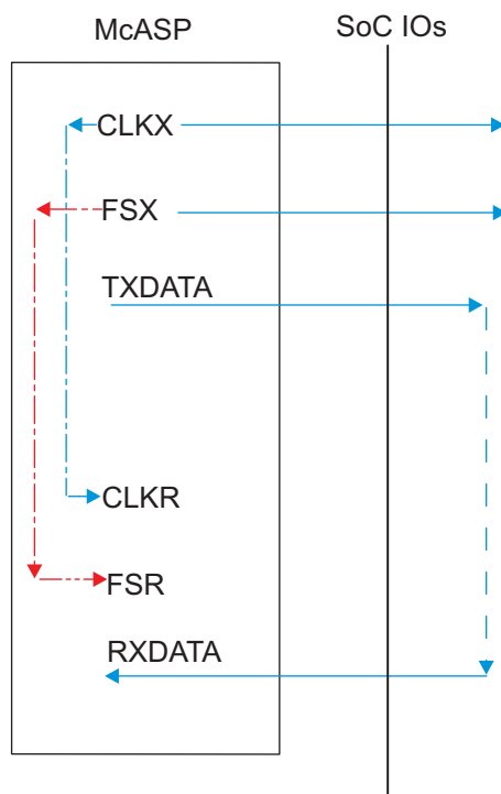
Figure 5-61. McASP1-8 CO-FO- – SYNC Mode
