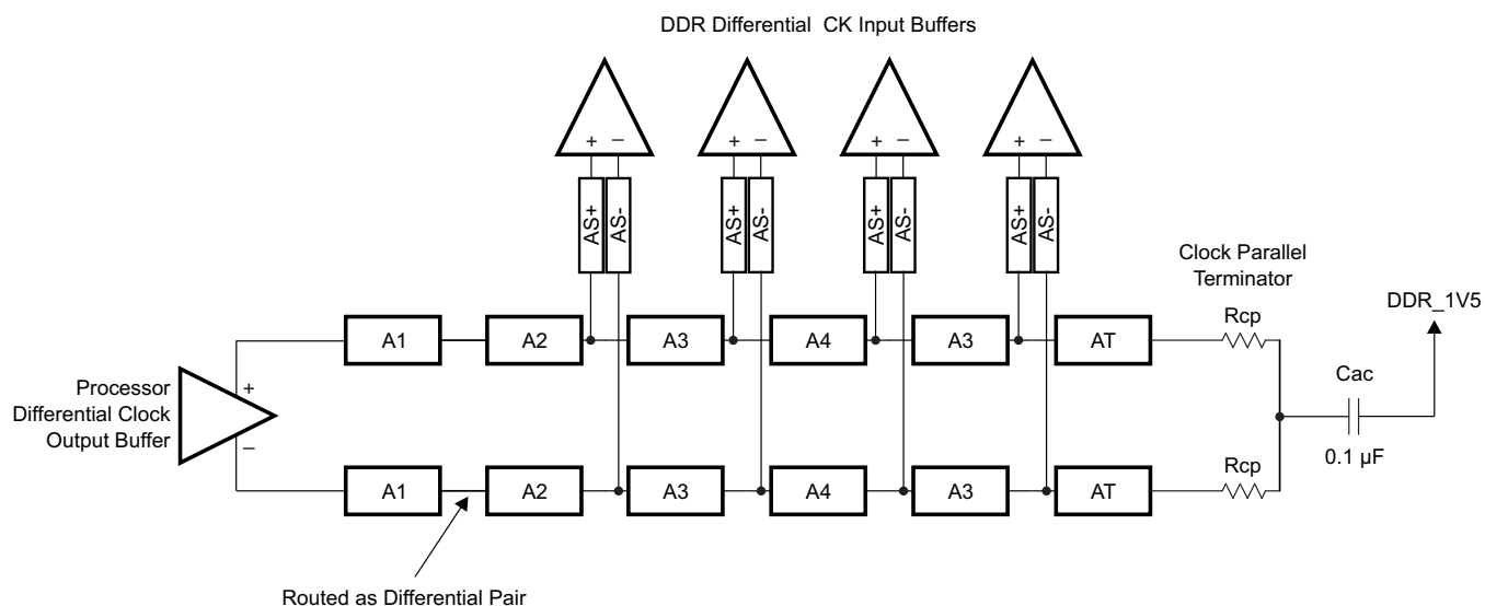
图 7-62. CK Topology for Four x8 DDR3 Devices
