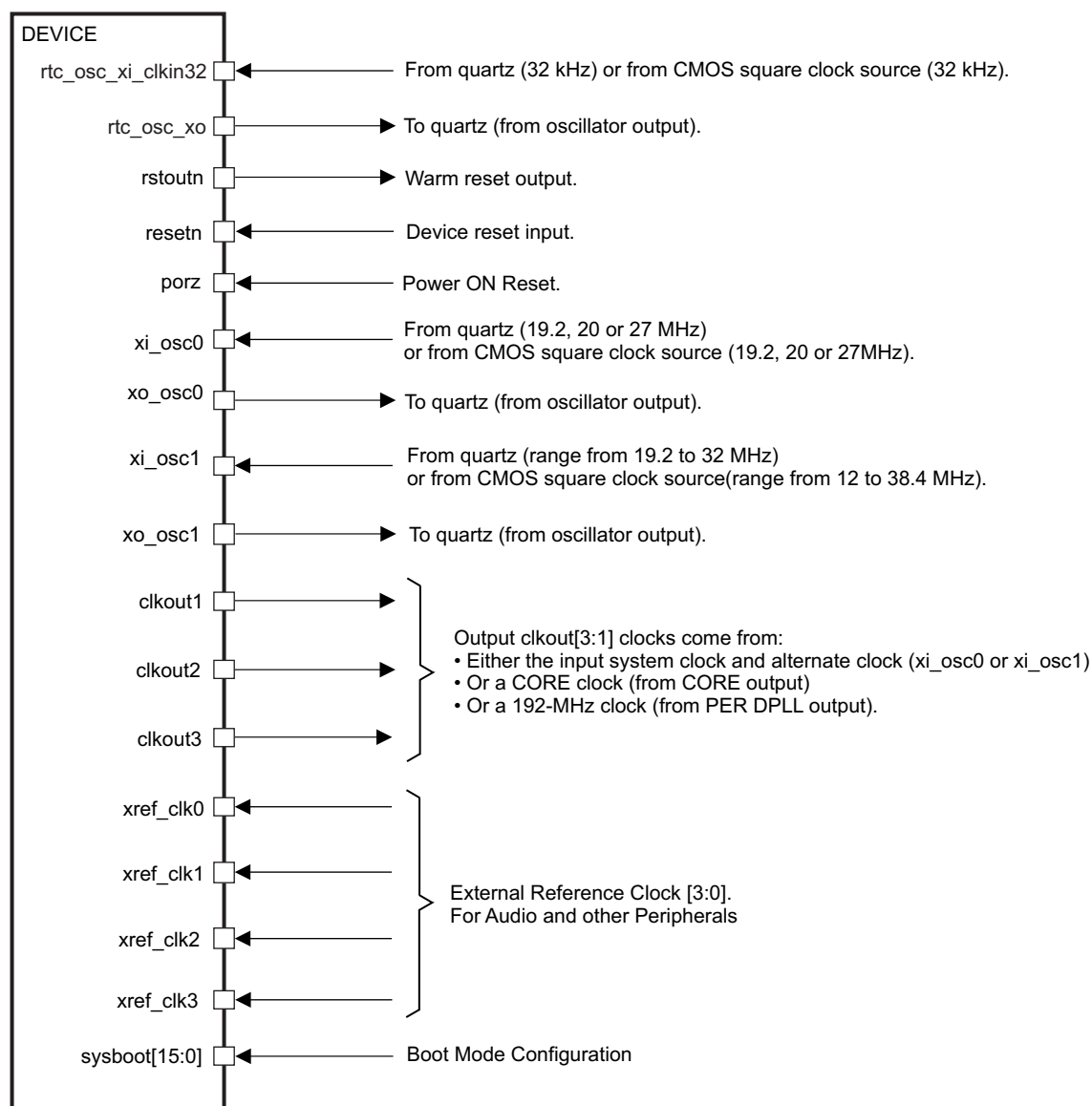
Figure 5-12. Clock Interface
