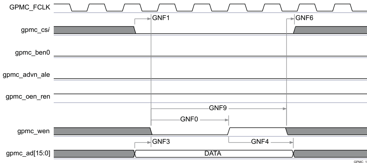
Figure 5-43. GPMC / NAND Flash - Data Write Cycle Timing (1)
