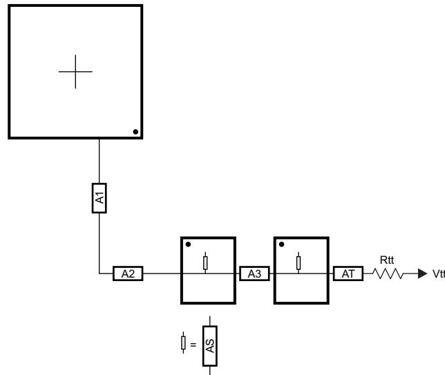
图 7-71. ADDR_CTRL Routing for Two Single-Side DDR3 Devices
