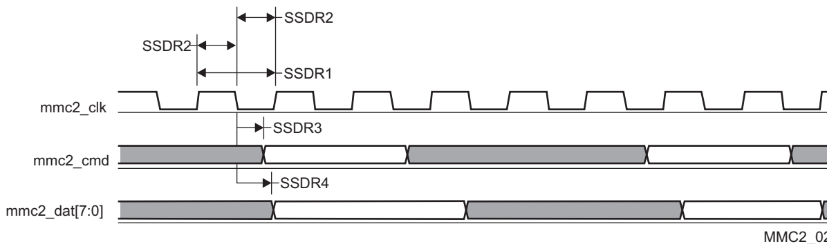
Figure 5-90. MMC/SD/SDIO in - Standard JC64 - Transmitter Mode
