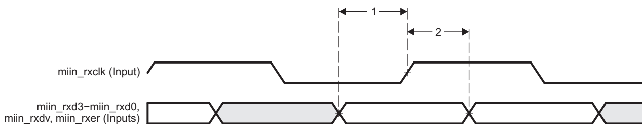
Figure 5-68. GMAC Receive Interface Timing MIIn Operation
