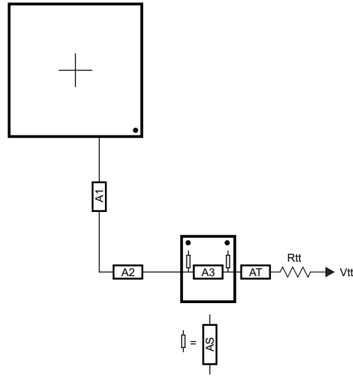
图 7-73. ADDR_CTRL Routing for Two Mirrored DDR3 Devices
