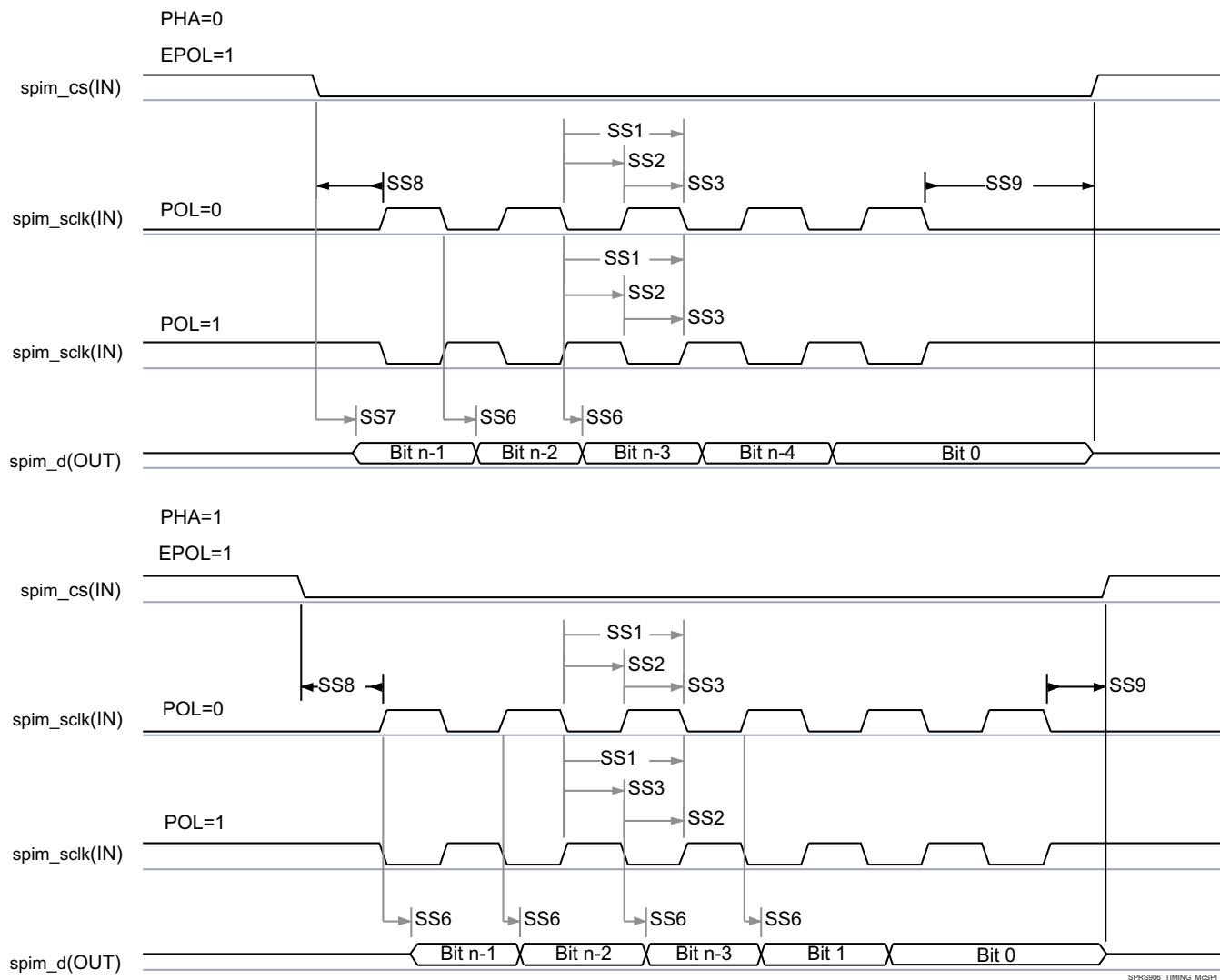
Figure 5-49. McSPI - Slave Mode Transmit
