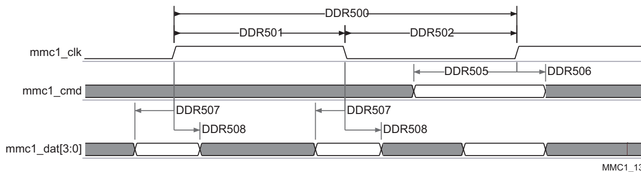
Figure 5-87. SDMMC - High Speed SD - DDR - Data/Command Receive
