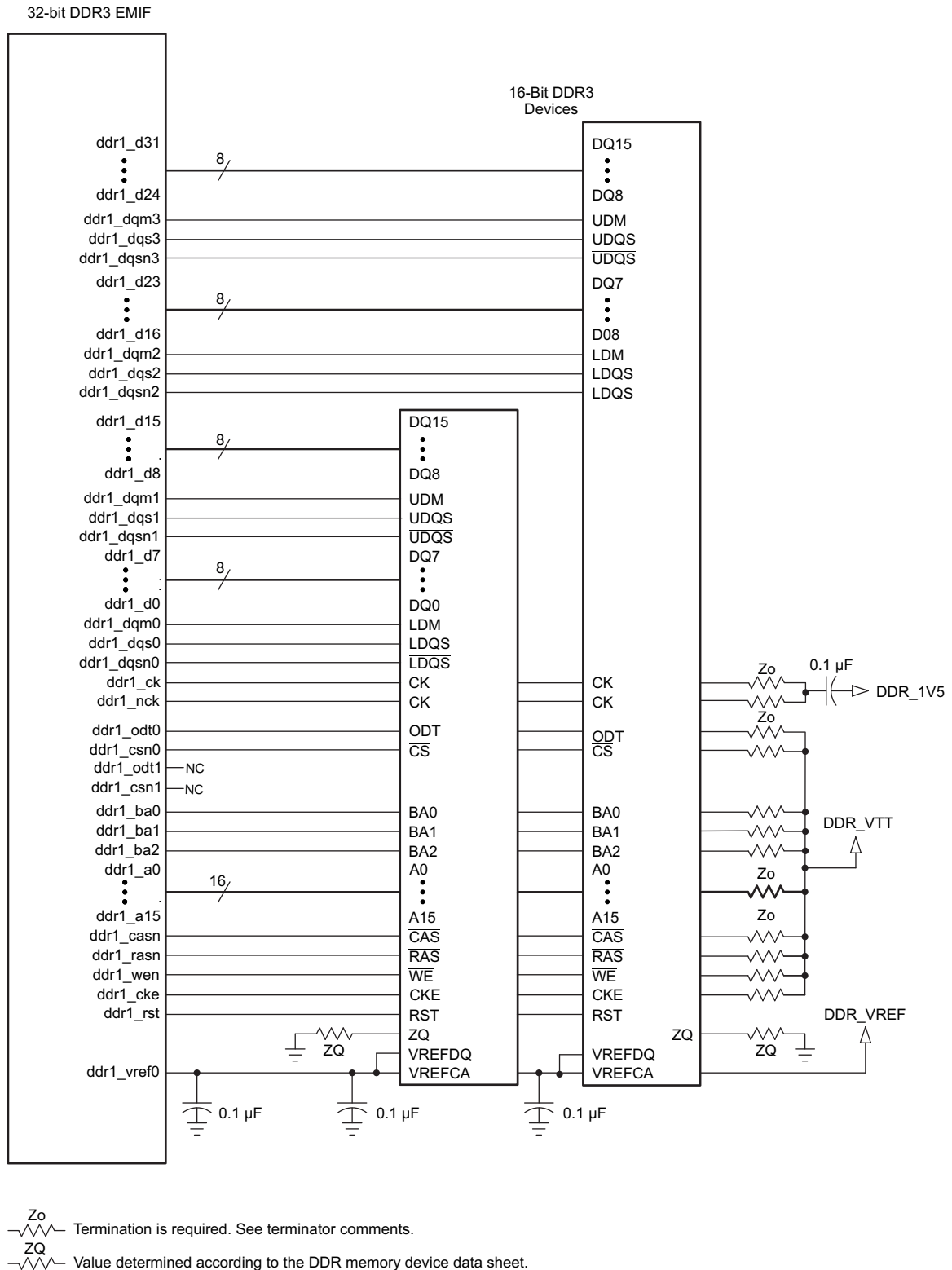
图 7-58. 32-Bit, One-Bank DDR3 Interface Schematic Using Two 16-Bit DDR3 Devices
