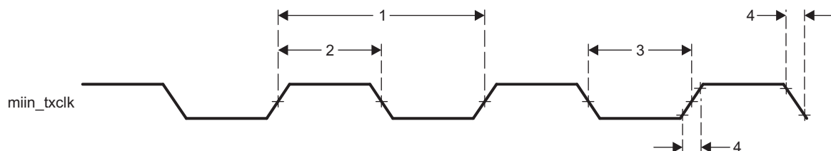
Figure 5-67. Clock Timing (GMAC Transmit) - MII Operation
