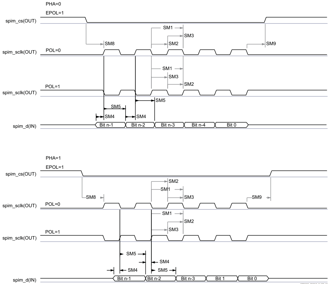
Figure 5-48. McSPI - Master Mode Receive
