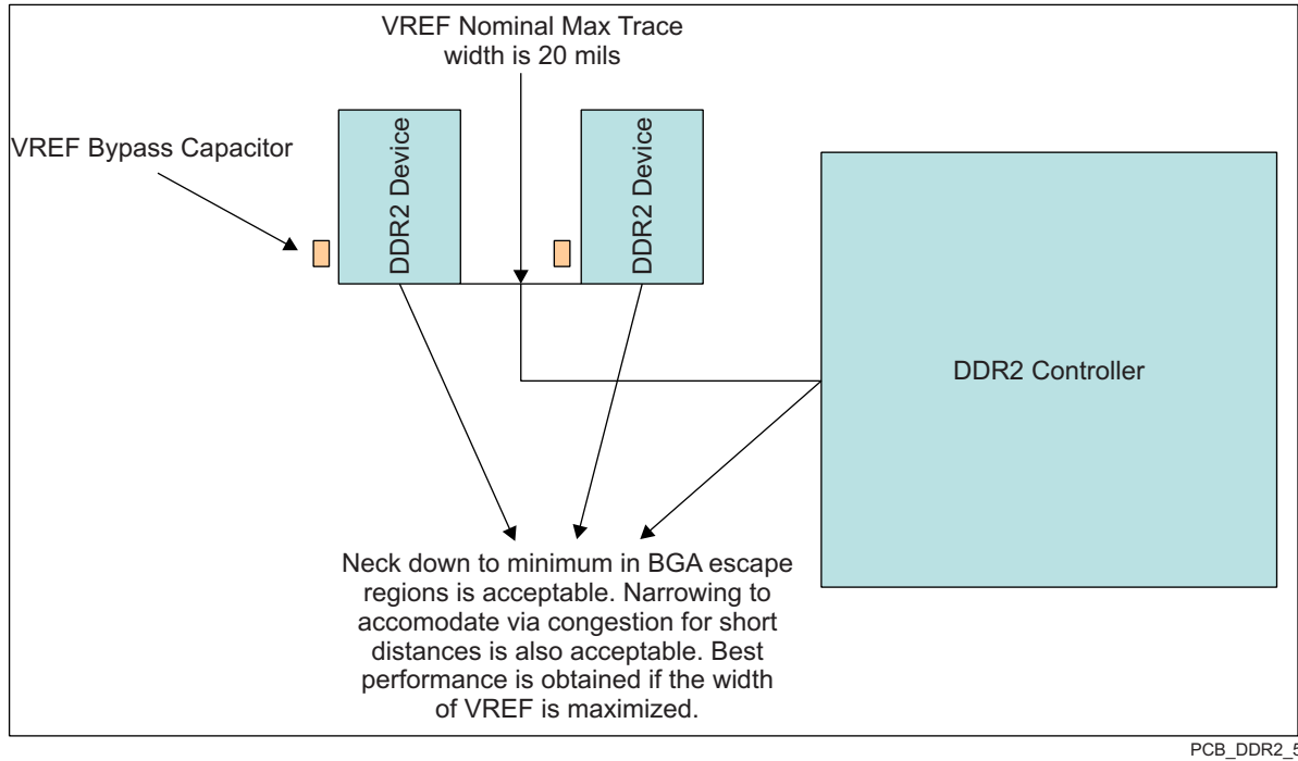
图 7-54. VREF Routing and Topology
