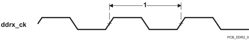
图 7-49. DDR2 Memory Controller Clock Timing
