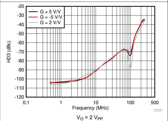
图 8-45. HD3 vs Frequency
