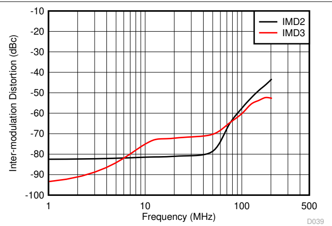
图 8-51. Intermodulation Distortion vs Frequency V_O = 2.5 V_{PP} per tone \pm 100\text{-kHz} frequency spacing
