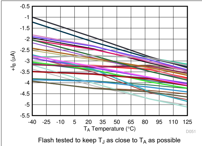
图 8-37. Noninverting I_B Over Temperature
