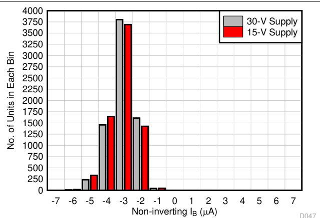
图 8-34. Noninverting I_B Distribution
