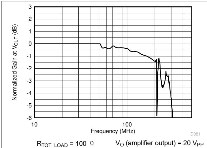
图 10-6. Frequency Response Of Two-Amplifier Configuration in 图 10-5 (Gain = 5 V/V, Measured At V OUT )
