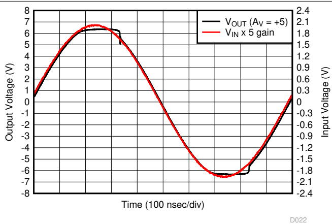
图 8-58. Overdrive Recovery Time
