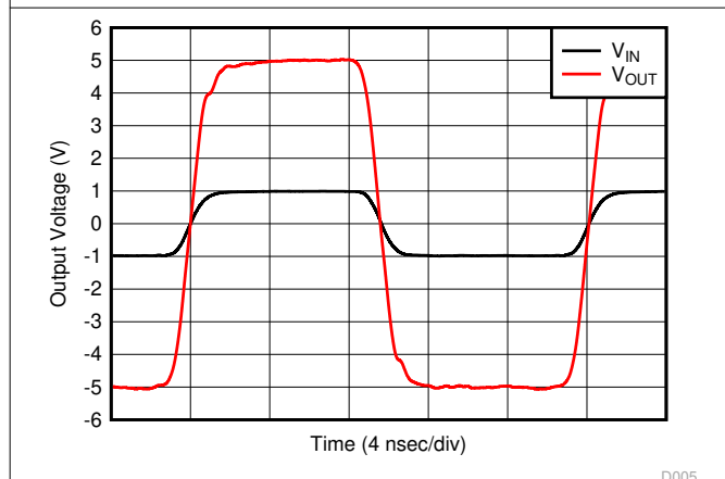
图 8-23. G = 5 V/V Pulse Response
