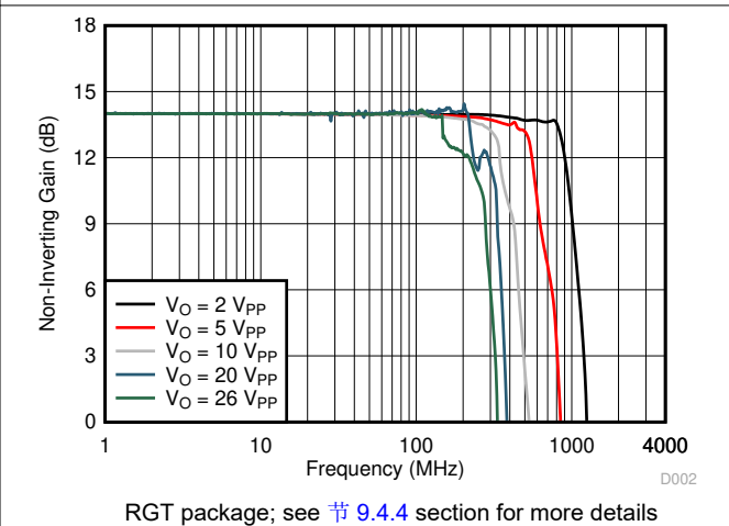
图 8-4. Frequency Response vs Output Swing
