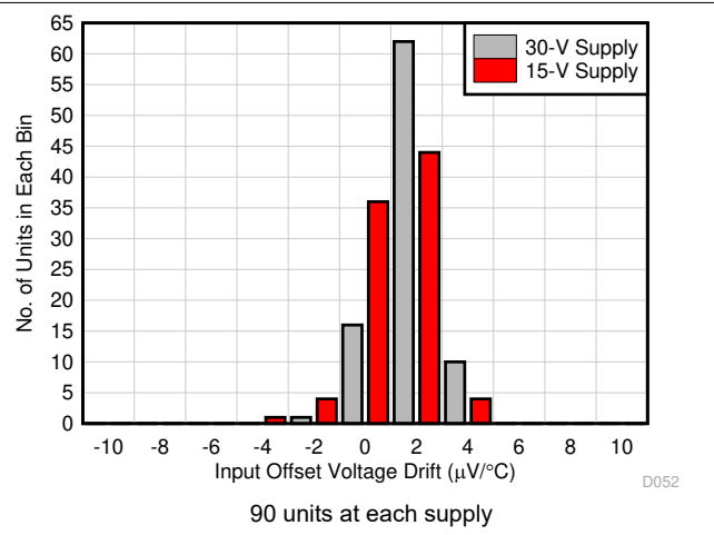
图 8-38. Input Offset Voltage Drift Histogram
