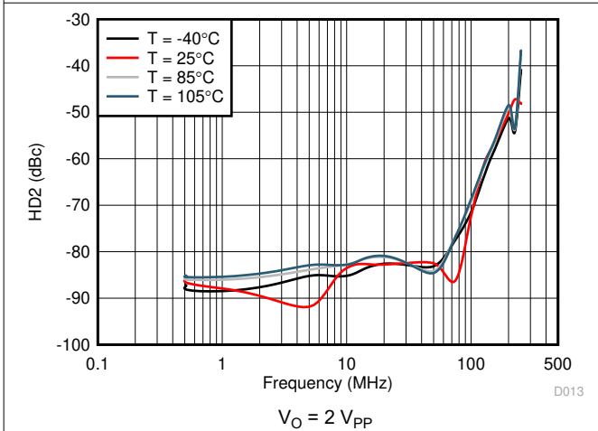
图 8-15. HD2 vs Frequency Across Temperature
