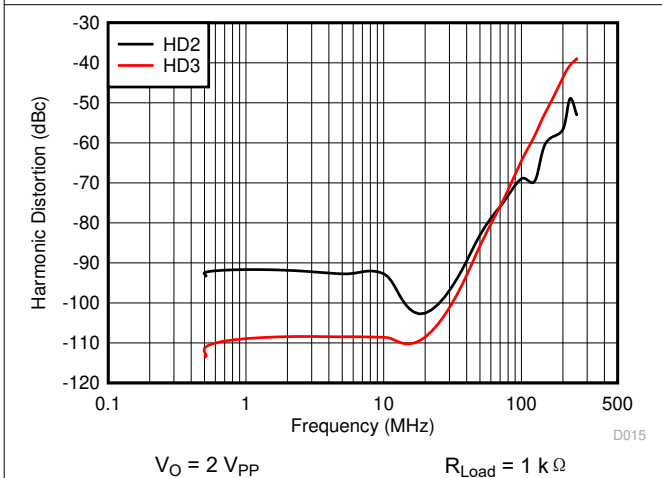
图 8-17. Harmonic Distortion vs Frequency
