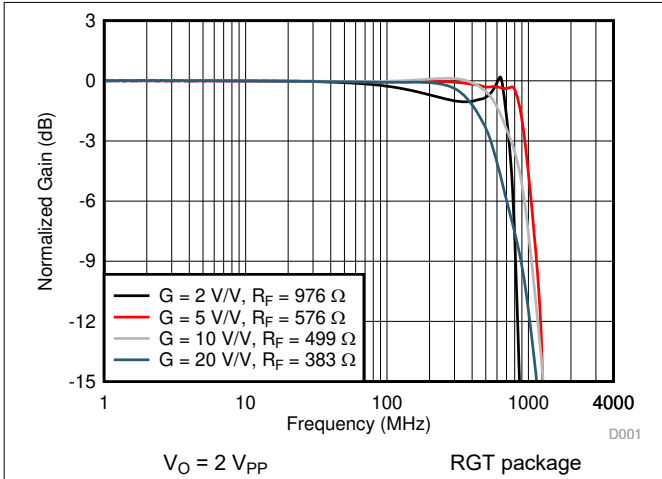
图 8-1. Noninverting Small-Signal Frequency Response
