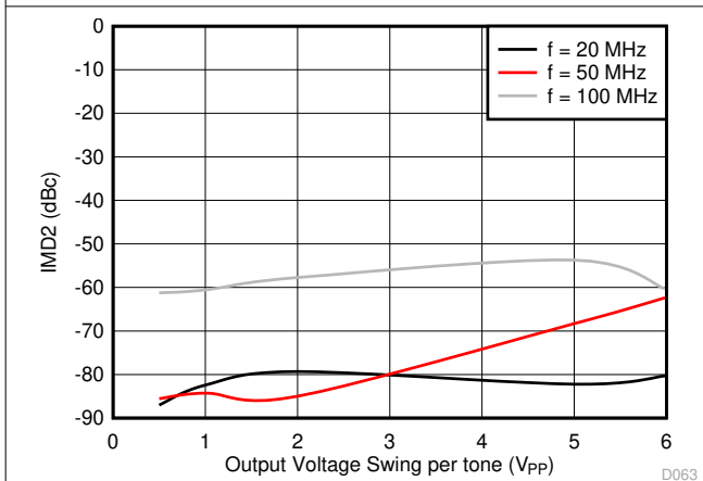
图 8-52. IMD2 vs Output Voltage Swing \pm 100\text{-kHz} frequency spacing
