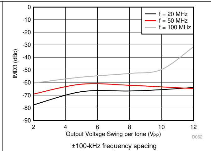
图 8-20. IMD3 vs Output Voltage Swing
