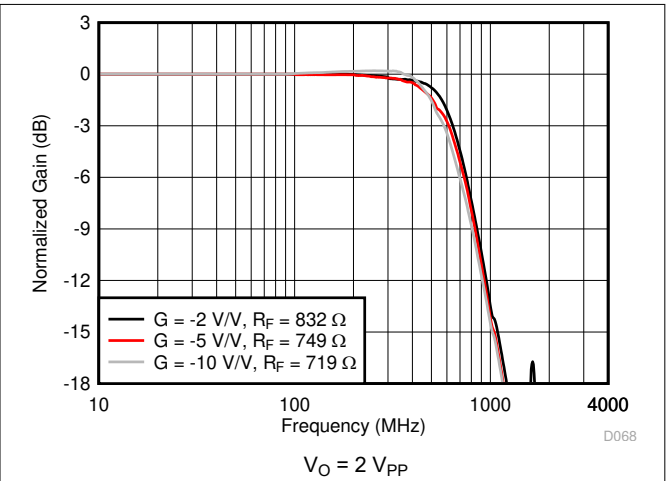
图 8-43. Inverting Small-Signal Frequency Response
