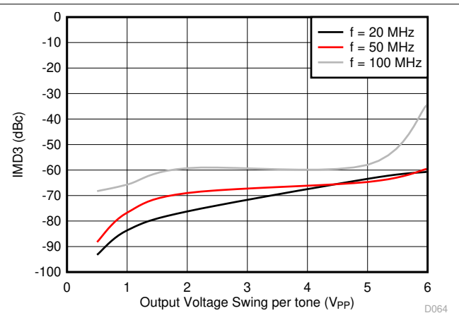
图 8-53. IMD3 vs Output Voltage Swing \pm 100\text{-kHz} frequency spacing
