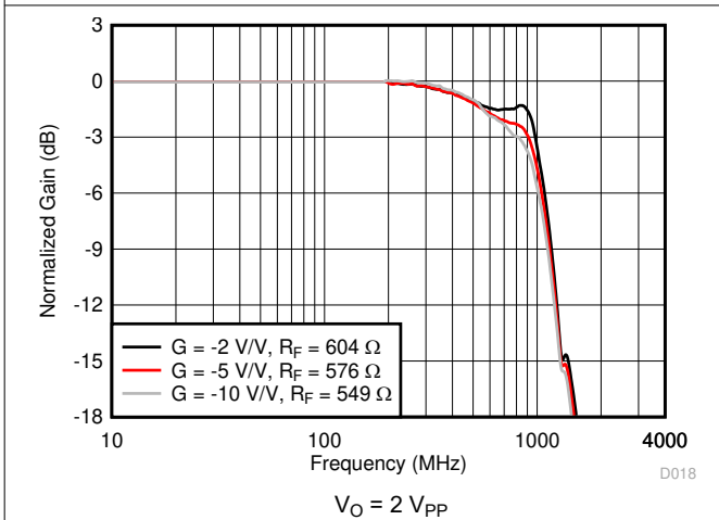
图 8-3. Inverting Small-Signal Frequency Response
