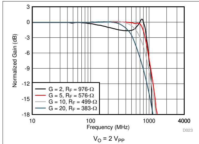
图 8-42. Noninverting Small-Signal Frequency Response
