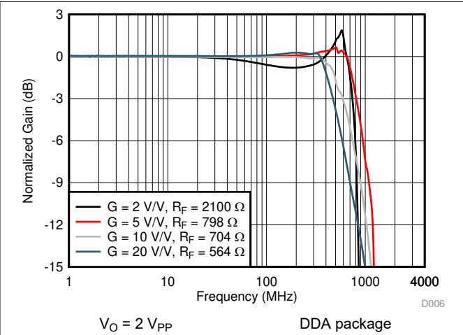
图 8-2. Noninverting Small-Signal Frequency Response
