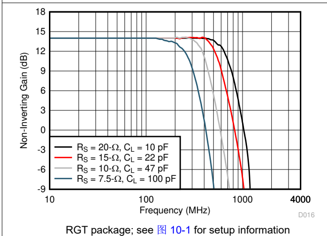
图 8-5. Frequency Response vs C_{LOAD}
