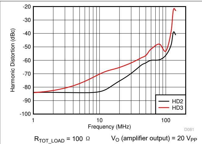
图 10-7. Distortion Of Two-Amplifier Configuration in 图 10-5 (Gain = 5 V/V, Measured At V OUT )
