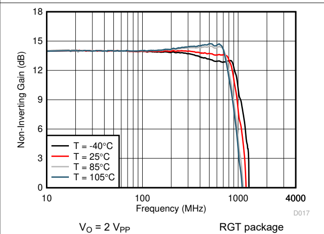
图 8-6. Frequency Response vs Temperature
