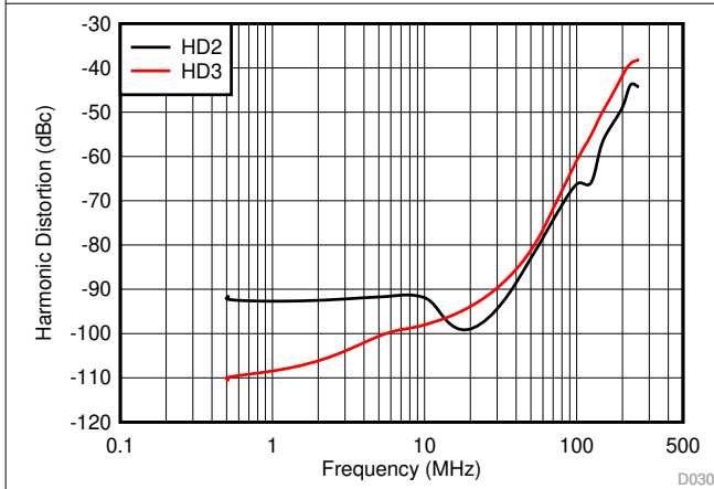
图 8-50. Harmonic Distortion vs Frequency V_O = 2 V_{PP} R_{LOAD} = 1 \text{ k}\Omega
