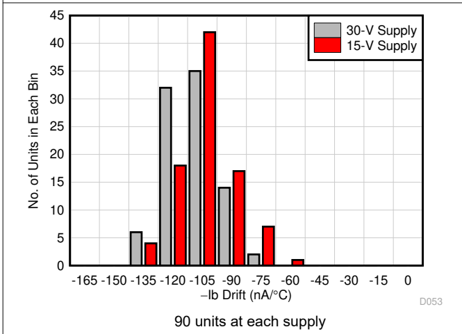
图 8-39. Inverting I_B Drift Histogram
