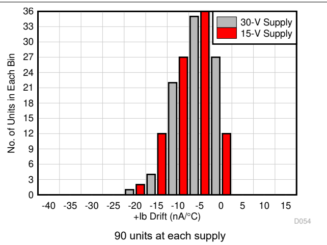
图 8-40. Noninverting I_B Drift Histogram
