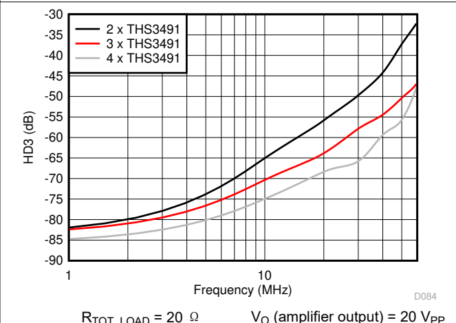
图 10-9. HD3 For Amplifier Load-Sharing Configuration (Gain = 5 V/V)
