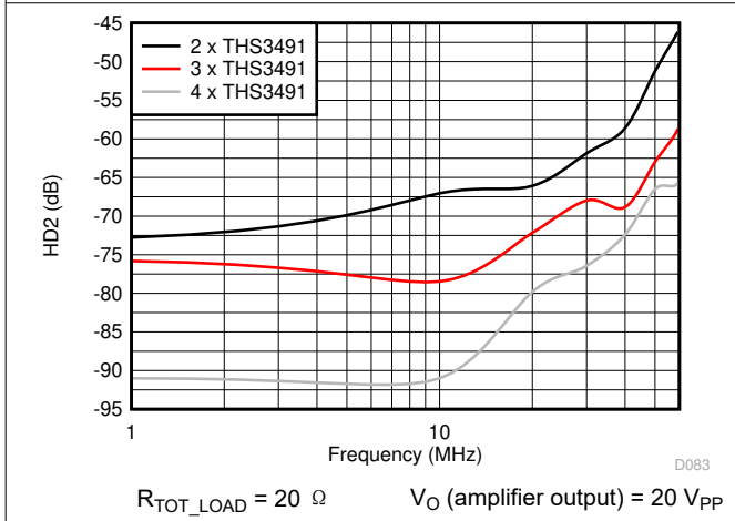
图 10-8. HD2 For Amplifier Load-Sharing Configuration (Gain = 5 V/V)
