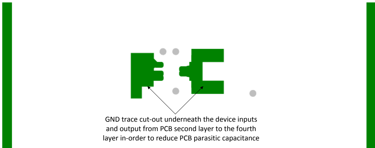
图 10-13. Ground Trace Cutout Beneath the Device Inputs and Output
