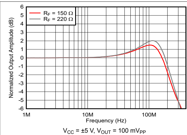
图 5-2. Frequency Response vs Feedback Resistance
