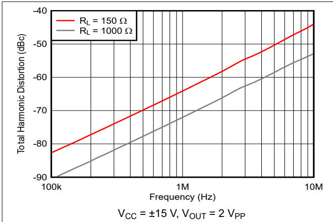
图 5-19. Total Harmonic Distortion vs Frequency
