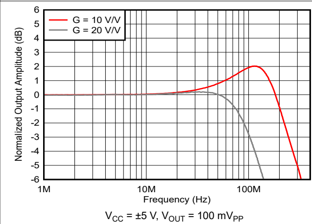
图 5-4. Frequency Response vs Gain
