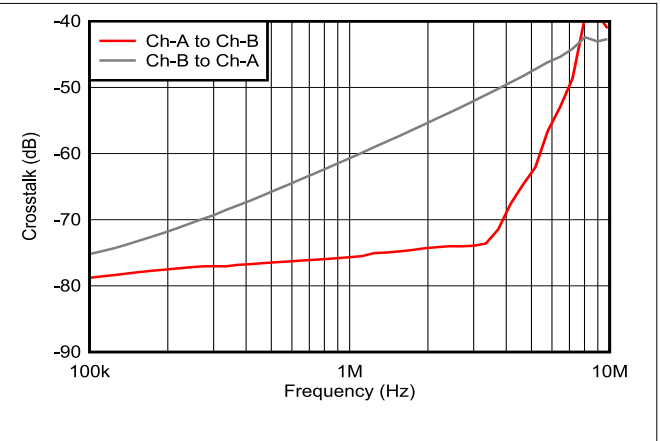
图 5-20. Crosstalk vs Frequency
