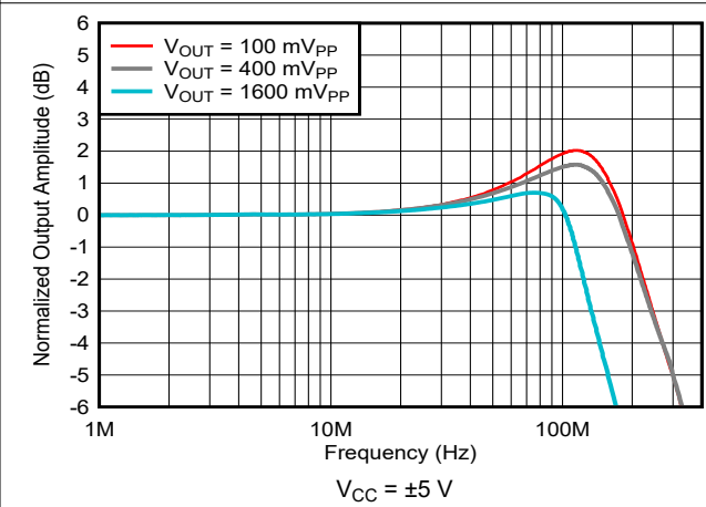
图 5-6. Large-Signal Frequency Response
