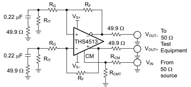
Figure 58. CM Input Test Circuit
