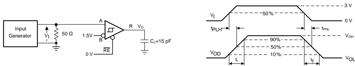
图 25. Measurement of Receiver Output Rise and Fall Times and Propagation Delays
