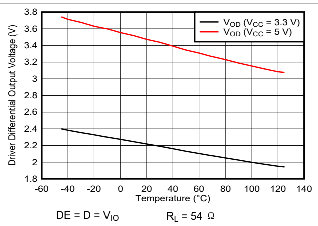
图 5-4. Driver differential output voltage vs Temperature
