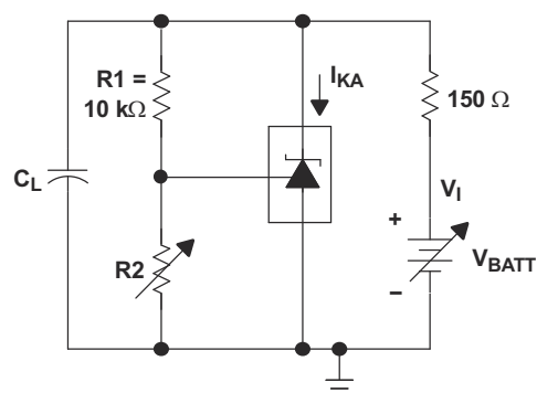
图 6-17. Test Circuits for Curves A Through D
