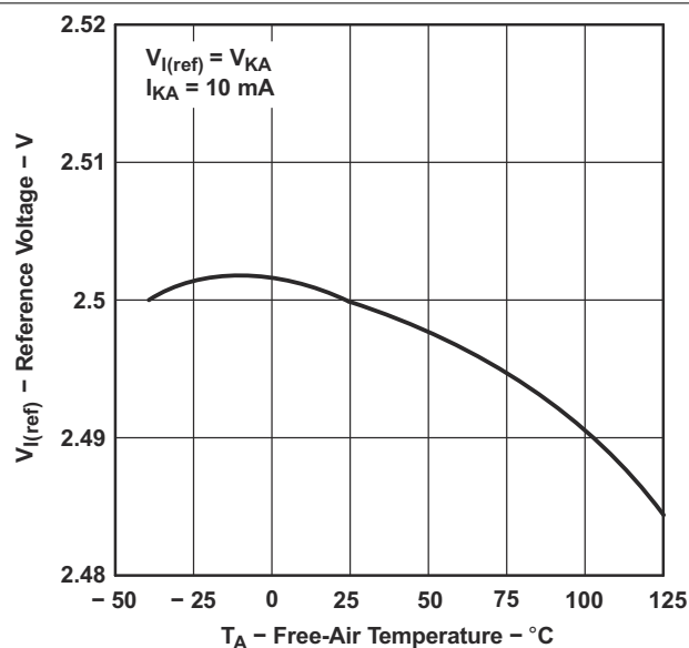
图 6-1. Reference Voltage vs Free-Air Temperature
