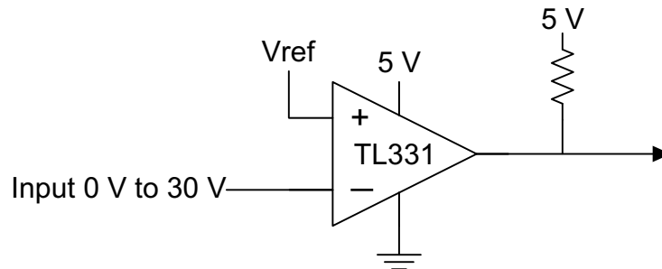
图 7-1. Typical Application Schematic
