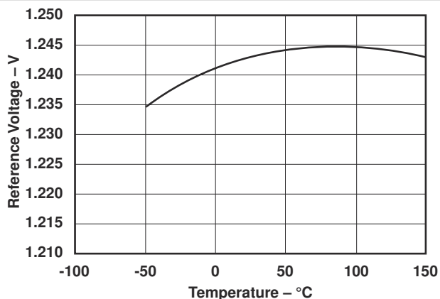
图 6-16. REFERENCE VOLTAGE vs TEMPERATURE
