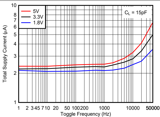
图 6-37. Supply Current vs. Toggle Frequency - Push-Pull Output
