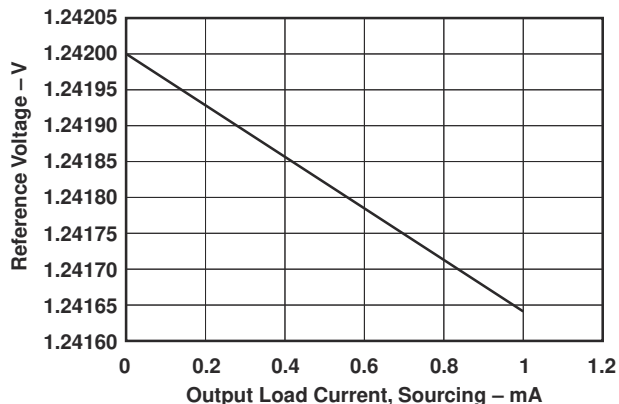
图 6-14. REFERENCE VOLTAGE vs OUTPUT LOAD CURRENT (SOURCING)
