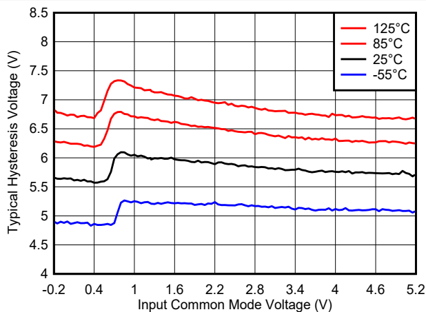
图 6-41. Hysteresis Voltage vs. Common Mode, 5V
