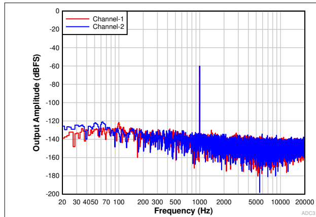
图 9-2. FFT With a -60-dBr Input
