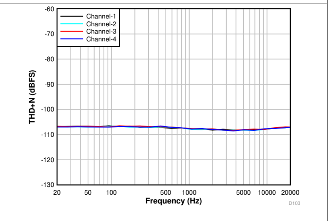
图 8. THD+N vs Input Frequency With a -60-dBr Input
