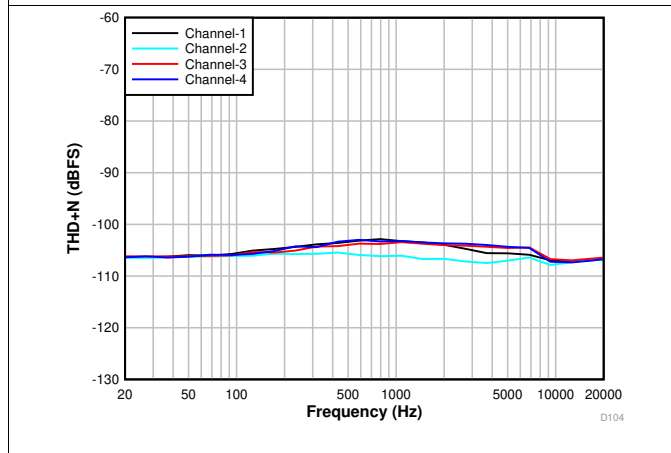
图 9. THD+N vs Input Frequency With a -1-dBr Input
