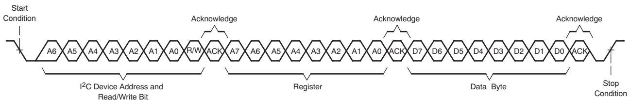
图 83. I 2 C Single-Byte Write Transfer
