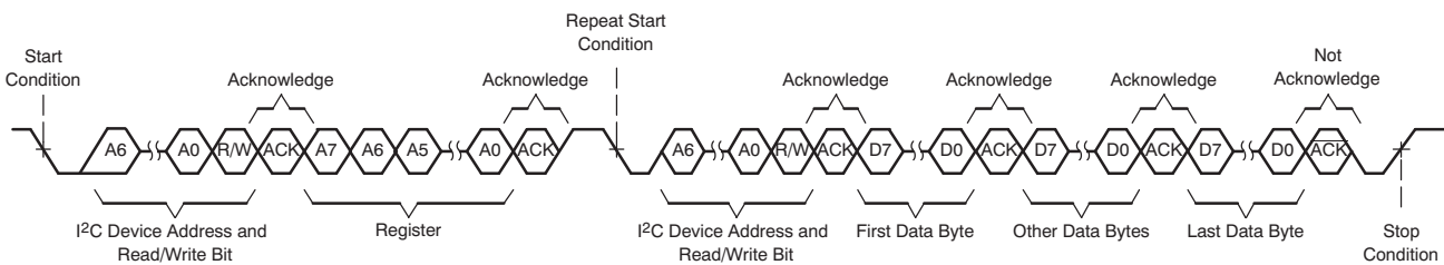
图 86. I 2 C Multiple-Byte Read Transfer
