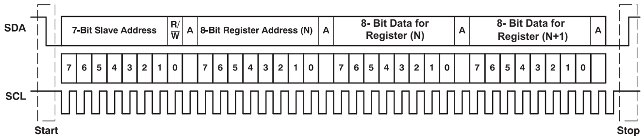
图 82. Typical I 2 C Sequence
