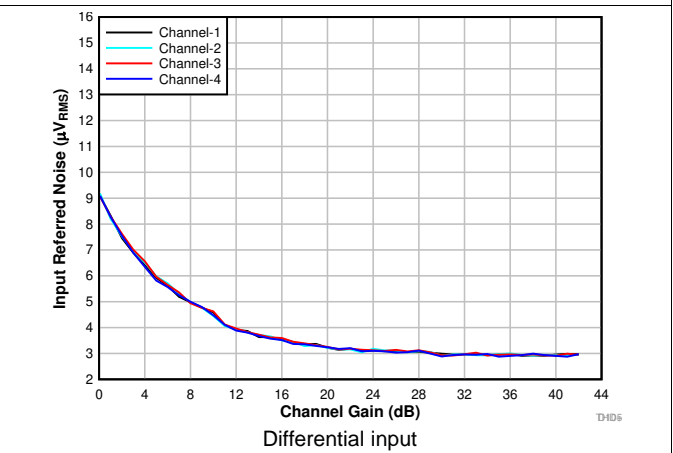
图 10. Input-Referred Noise vs Channel Gain
