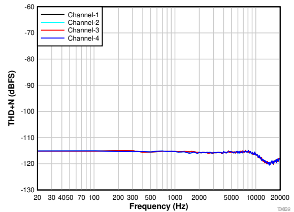
图 7-25. PDM Input THD+N vs Input Frequency With a -20-dBr Input
