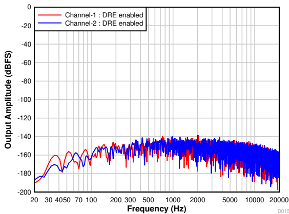
图 7-18. FFT With Idle Input With DRE Enabled
