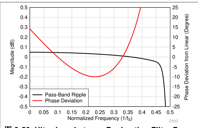
图 8-50. Ultra-Low-Latency Decimation Filter Pass-Band Ripple and Phase Deviation
