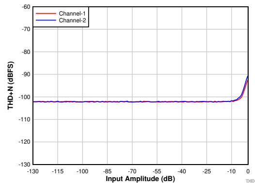
图 7-7. THD+N vs Input Amplitude With DRE Disabled
