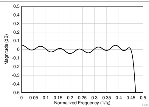
图 8-30. Linear Phase Decimation Filter Pass-Band Ripple
