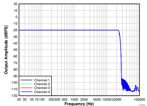
图 7-27. PDM Input Frequency Response With a -20-dBr Input
