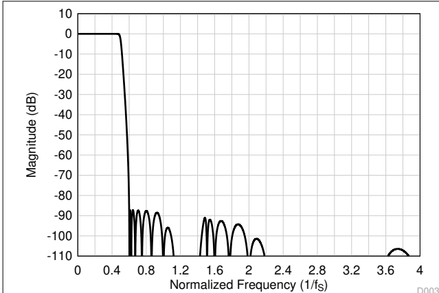
图 8-51. Ultra-Low-Latency Decimation Filter Magnitude Response
