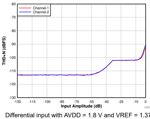
图 7-8. THD+N vs Input Amplitude With DRE Enabled
