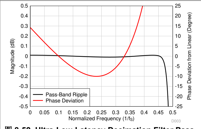
图 8-52. Ultra-Low-Latency Decimation Filter Pass-Band Ripple and Phase Deviation
