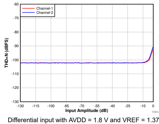
图 7-9. THD+N vs Input Amplitude With DRE Disabled
