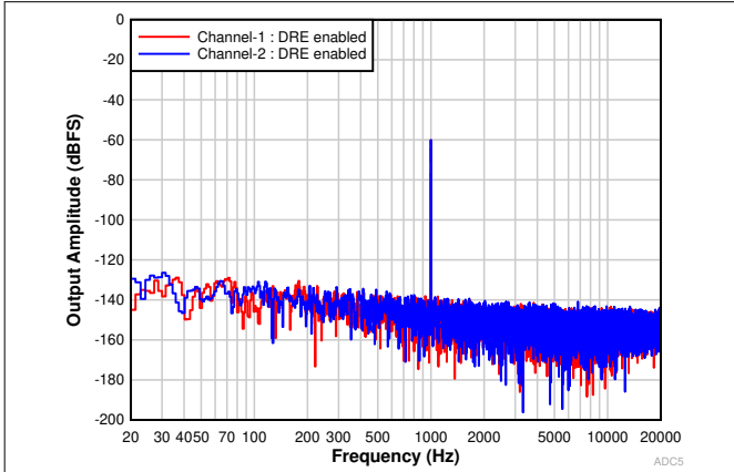
图 9-2. FFT With a -60-dBr Input With DRE Enabled
