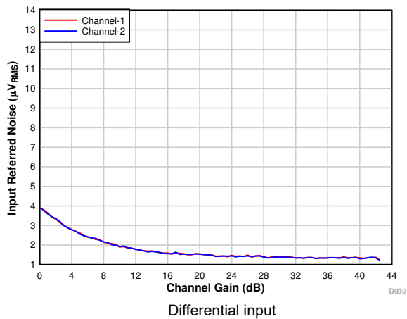
Figure 7-13. Input-Referred Noise vs Channel Gain
