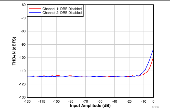
图 9-5. THD+N vs Input Amplitude With DRE Disabled
