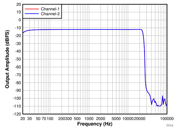
Figure 7-15. Frequency Response With a -12\text{-dBr} Input
