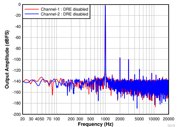
图 7-21. FFT With a -1-dBr Input With DRE Disabled
