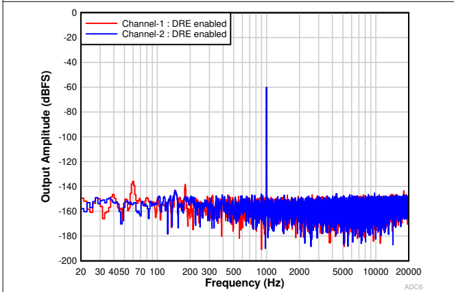
图 9-4. FFT With a -60-dBr Input With DRE Disabled
