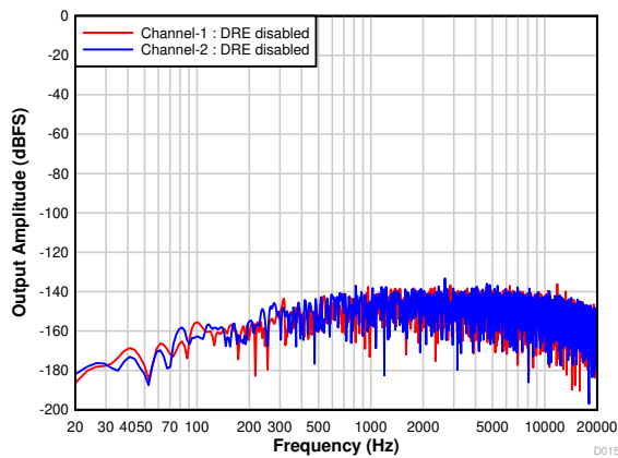
图 7-18. FFT With Idle Input With DRE Disabled
