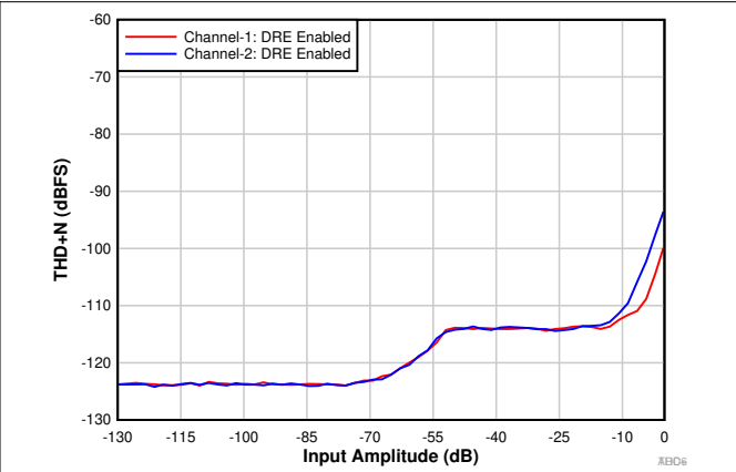
图 9-3. THD+N vs Input Amplitude With DRE Enabled
