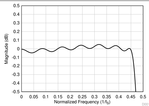
图 8-22. Linear Phase Decimation Filter Pass-Band Ripple
