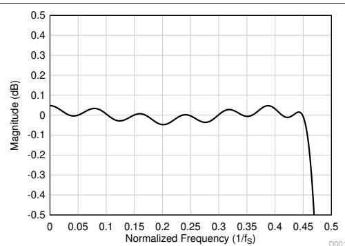
图 8-24. Linear Phase Decimation Filter Pass-Band Ripple
