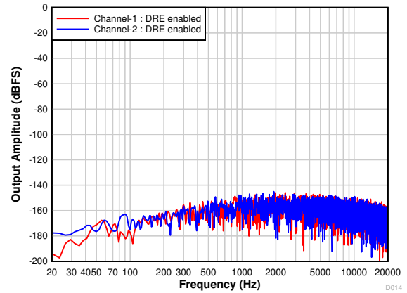
图 7-17. FFT With Idle Input With DRE Enabled
