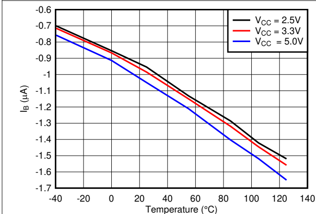
图 5-5. Bias Current vs Temperature
