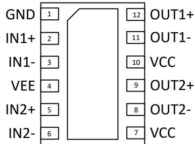
图 5-3. WSON Package 12-Pin DSS Top View
