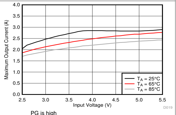
图 16. Maximum Output Current at V_OUT = 1.8 V
