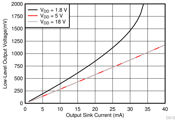
图 7-10. Output Voltage Low ( V_{OL} ) vs Output Sink Current ( 0^\circ\text{C} )
