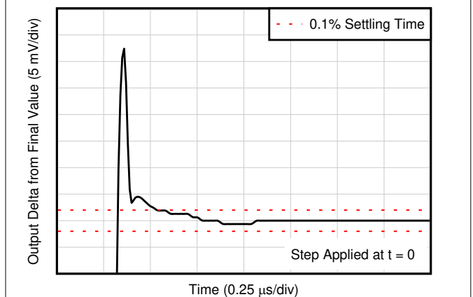
C_L = 20\text{pF} , 增益 = -1, V_{IN} = 2\text{V} 阶跃
