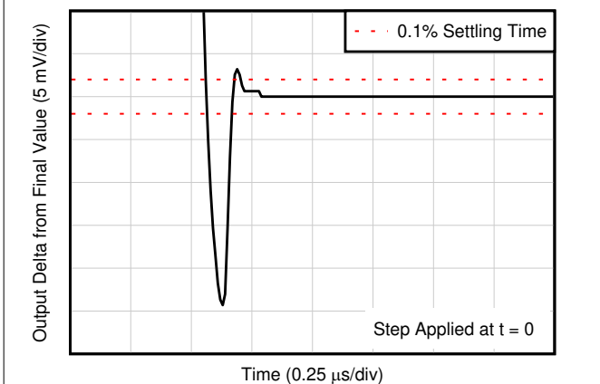
C_L = 20\text{pF} , 增益 = 1, V_{IN} = 2\text{V} 阶跃
