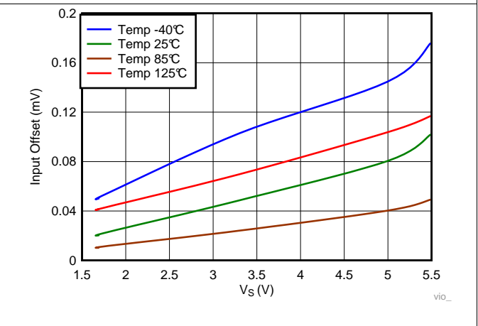
Figure 12. Input Offset vs. V_S
