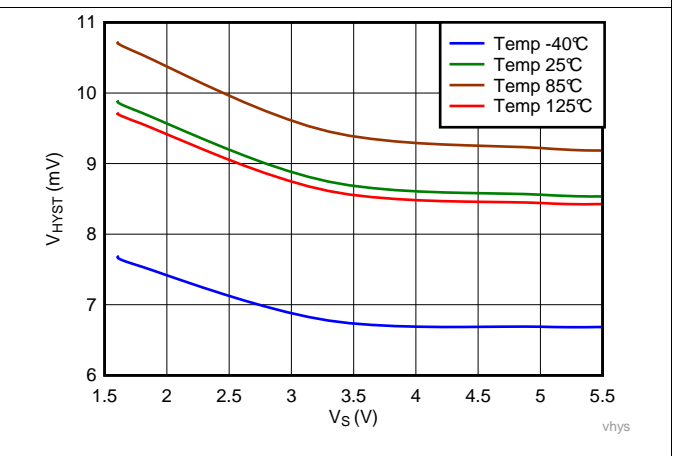
Figure 14. Hysteresis vs V_S
