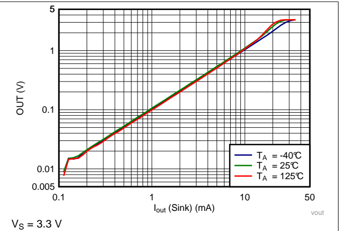
Figure 10. Output Voltage Low vs. Output Sink Current
