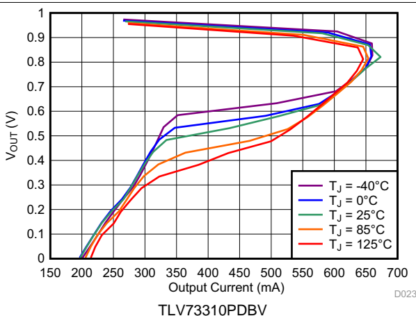
Figure 18. 1.0-V Foldback Current Limit vs I_{OUT} and Temperature
