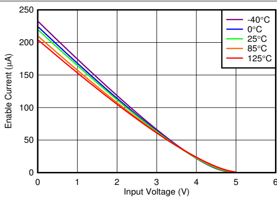
V_{EN} = 5.5\text{V}
