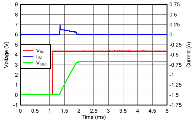
图 5-20. Inrush Current With 22\ \mu\text{F} at C_{OUT}
