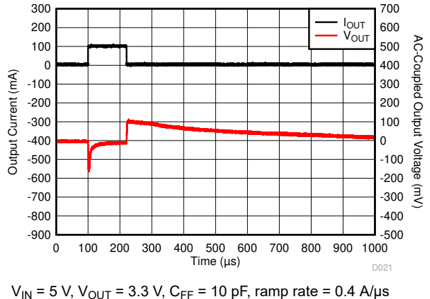
图 6-10. I_{OUT} Transient From 0\text{ mA} to 100\text{ mA}
