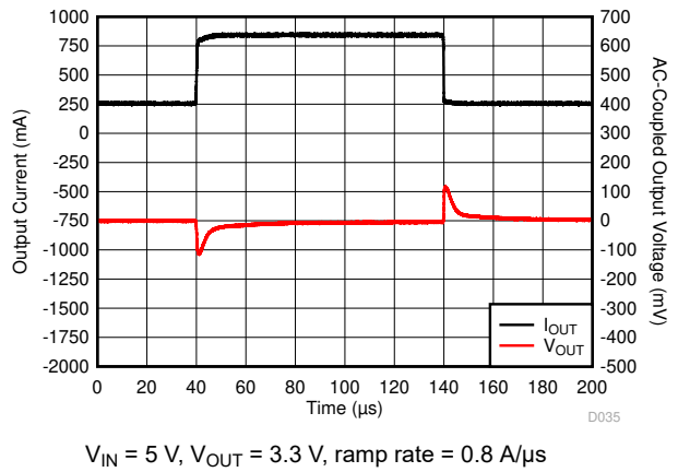
图 6-12. I_{OUT} Transient From 250\text{ mA} to 850\text{ mA}
