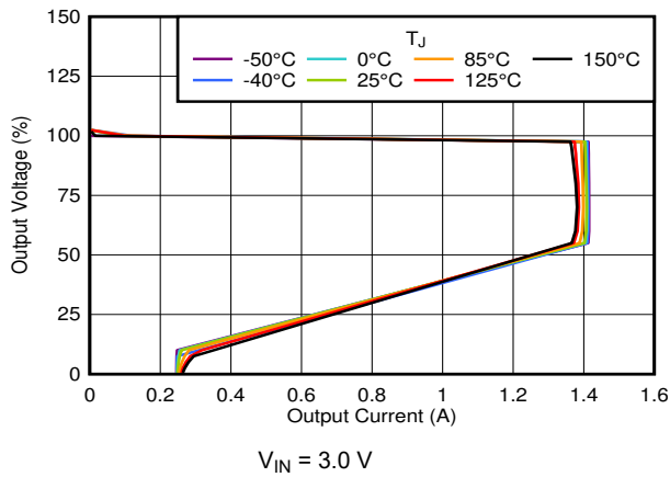
图 6-19. Foldback Current Limit vs I_{OUT} and Temperature
