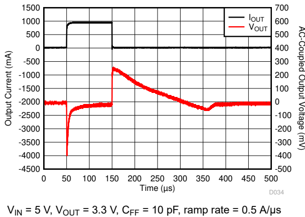
图 6-11. I_{OUT} Transient From 1\text{ mA} to 1\text{ A}
