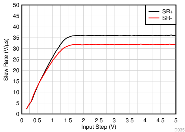
G = +1, C_L = 20\text{pF}
