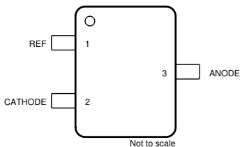
图 4-4. TLVH431 DBZ Package 3-Pin SOT-23 Top View
