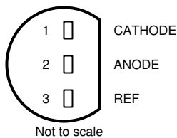
图 4-3. TLVH431 LP Package 3-Pin TO-92 Top View
