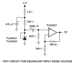
TEST CIRCUIT FOR EQUIVALENT INPUT NOISE VOLTAGE
