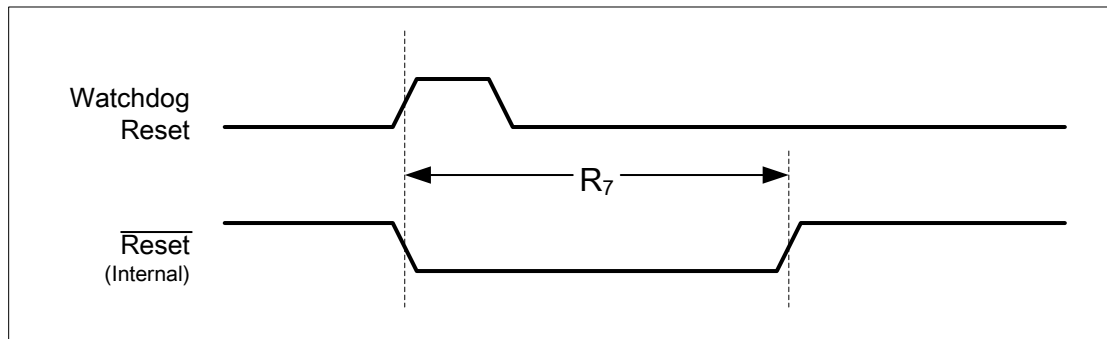
图 24-13. Watchdog Reset Timing
