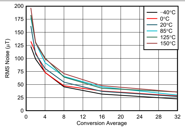
图 5-4. X, Y-Axis Noise vs Conversion Average, 50-mT Range
