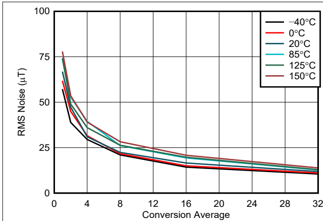
图 5-7. Z-Axis Noise vs Conversion Average, 100-mT Range
