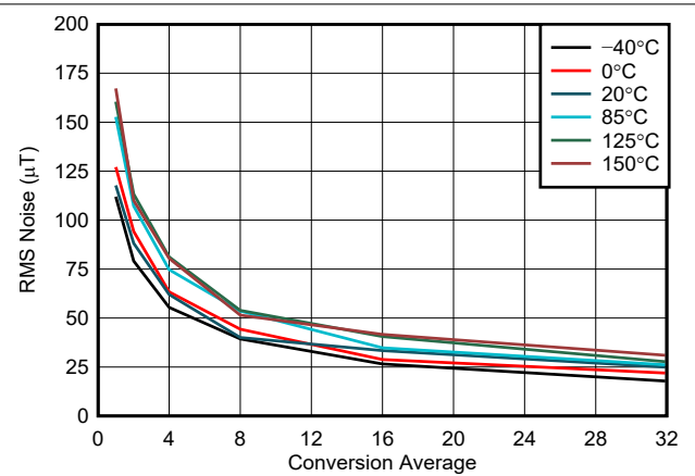
图 5-2. X, Y-Axis Noise vs Conversion Average, 25-mT Range
