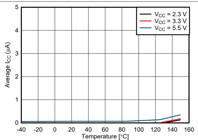
图 5-18. Deep Sleep Mode Supply Current vs Temperature
