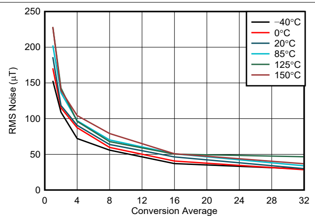
图 5-12. X, Y-Axis Noise vs Conversion Average, 300-mT Range
