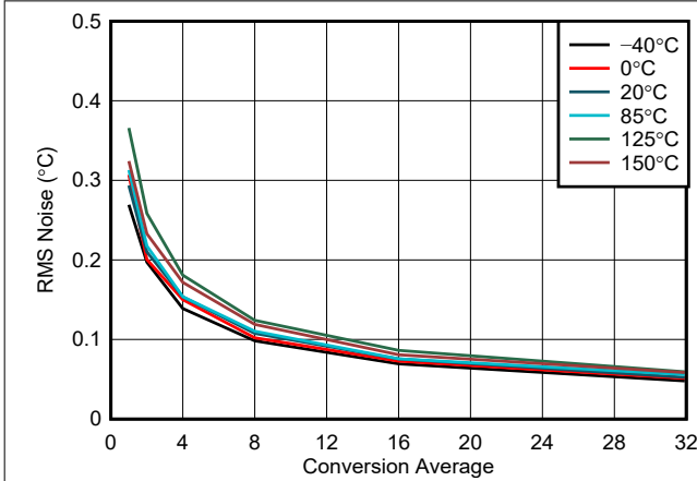
图 5-13. Temperature Sensor Noise vs Conversion Average
