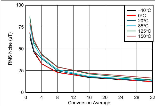
图 5-3. Z-Axis Noise vs Conversion Average, 50-mT Range
