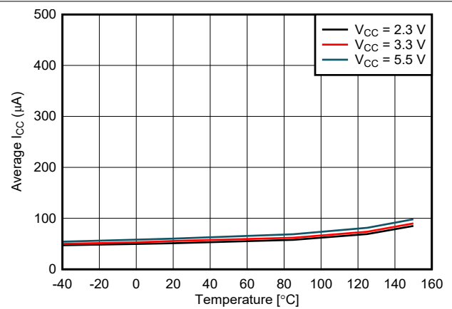
图 5-16. Configuration Mode Supply Current vs Temperature
