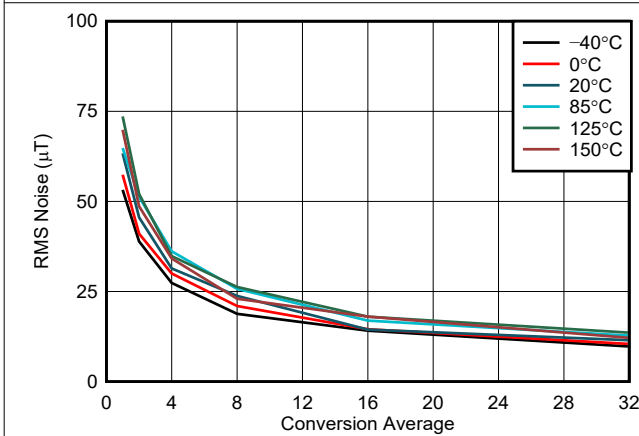
图 5-5. Z-Axis Input vs Conversion Average, 75-mT Range
