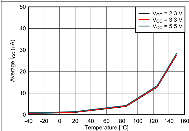
图 5-17. Sleep Mode Supply Current vs Temperature
