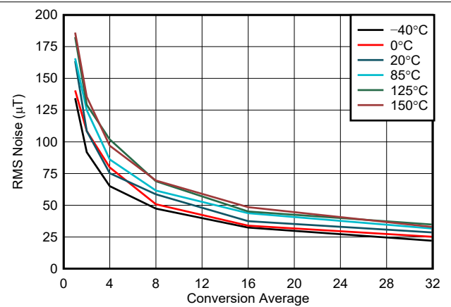
图 5-6. X, Y-Axis Noise vs Conversion Average, 75-mT Range
