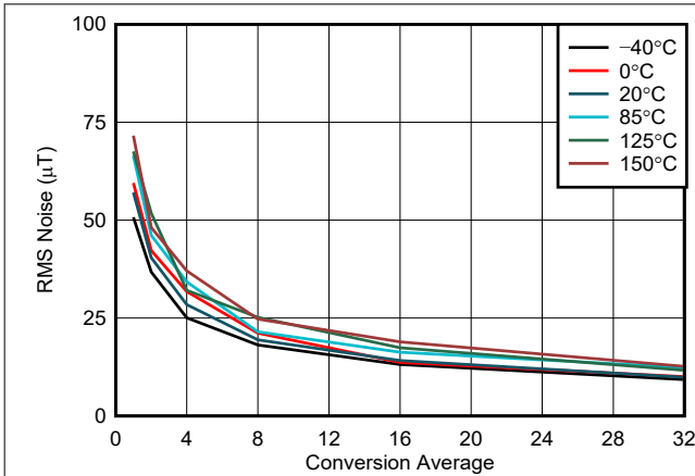
图 5-1. Z-Axis Noise vs Conversion Average, 25-mT Range
