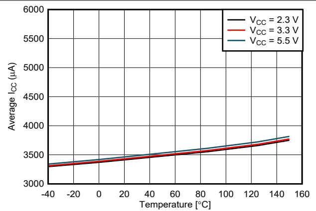
图 5-14. Active Mode Supply Current vs Temperature
