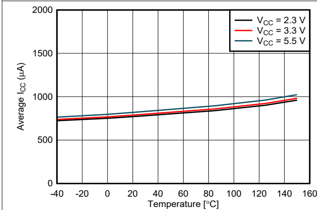
图 5-15. Standby Mode Supply Current vs Temperature
