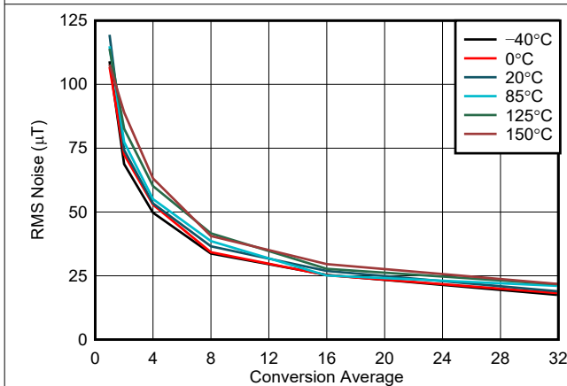
图 5-11. Z-Axis Noise vs Conversion Average, 300-mT Range
