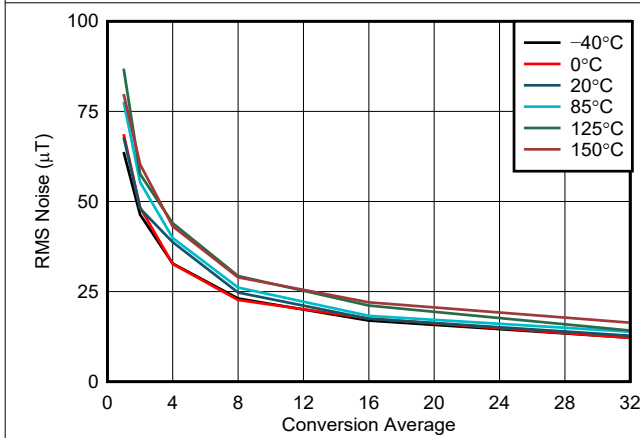
图 5-9. Z-Axis Noise vs Conversion Average, 150-mT Range
