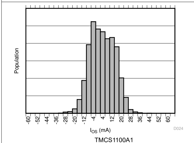
图 7-5. Input Offset Current Production Distribution
