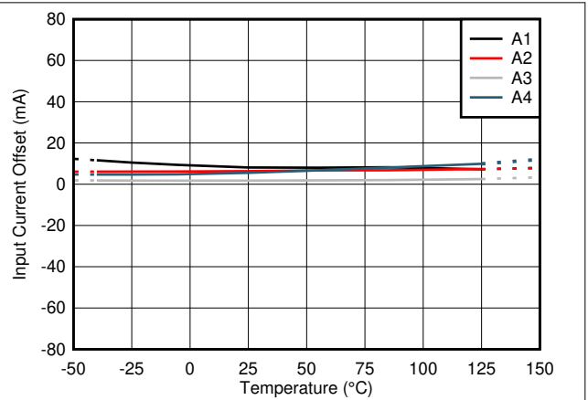
图 7-2. Input Offset Current vs. Temperature
