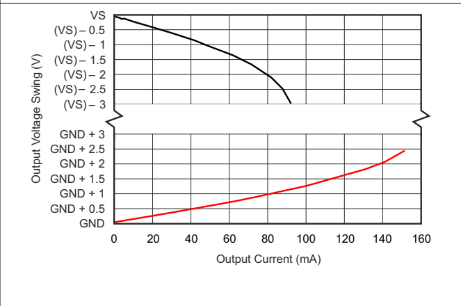
图 7-12. Output Swing vs. Output Current
