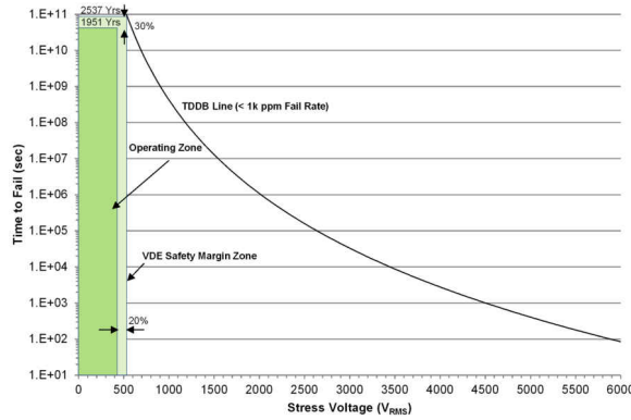
图 9-1. Insulation Lifetime
