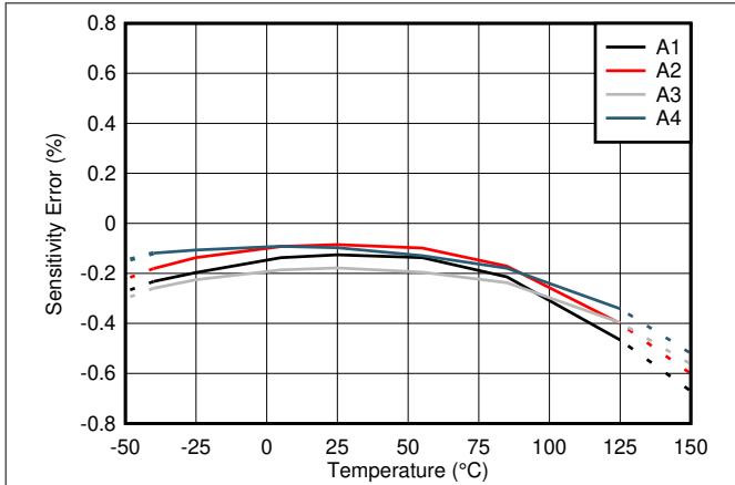
图 7-1. Sensitivity Error vs. Temperature
