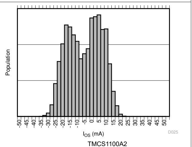
图 7-6. Input Offset Current Production Distribution
