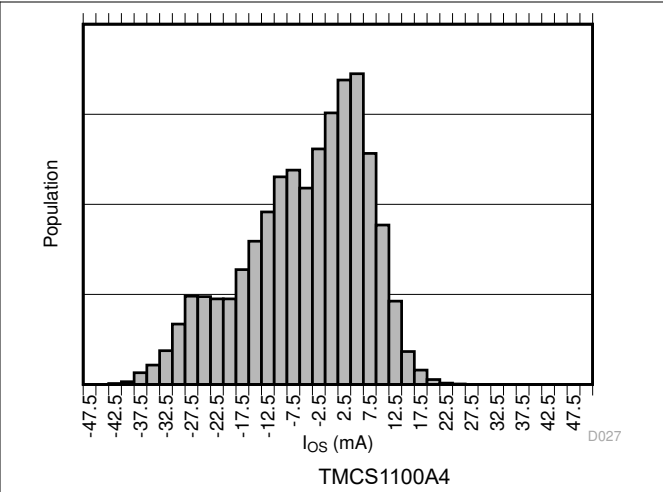
图 7-8. Input Offset Current Production Distribution
