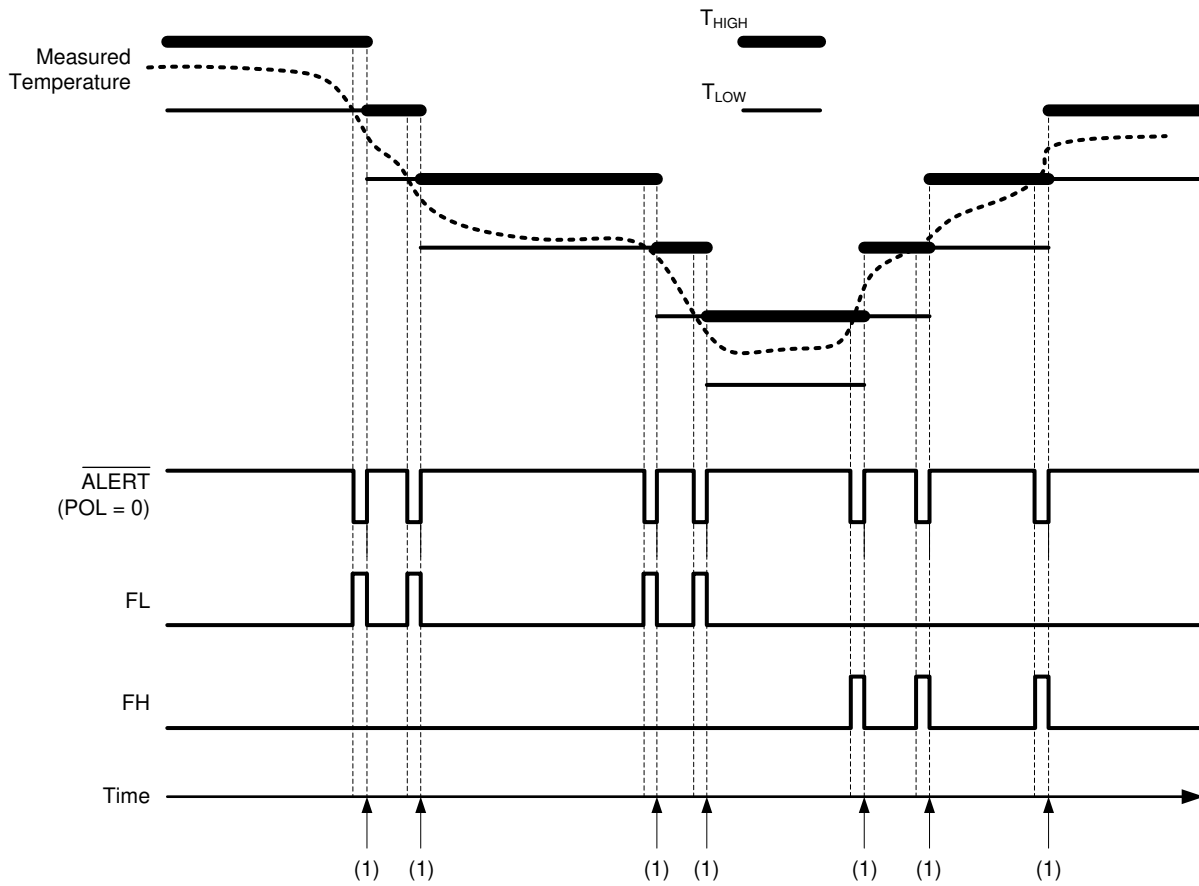
Figure 13. Interrupt Mode
