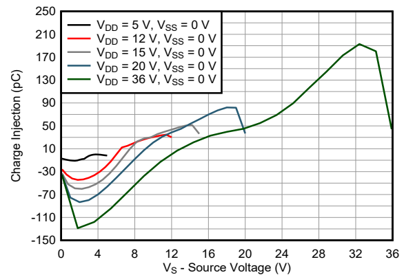
图 6-16. Charge Injection vs Source Voltage - Single Supplies
